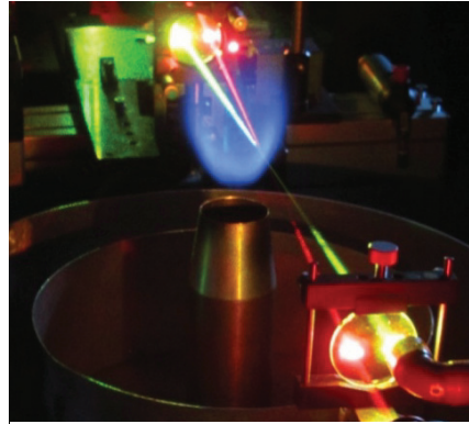
Figure 4.17. Photograph of rotational CARS measurements in a low-swirl turbulent premixed flame.
