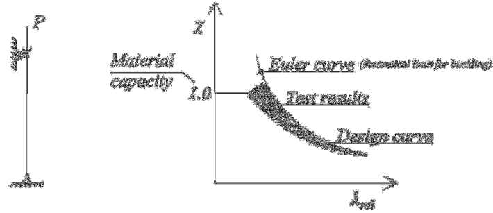
Figure 3.1: A schematic diagram of a typical design curve for the design of columns: \lambda_{rel} = \sqrt{N_p / N_{cr}} and P_u = \chi N_p . N_p being the plastic capacity of the column, N_{cr} the Euler buckling load, and P_u the "capacity" of the column.
