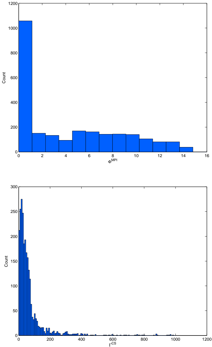
FIGURE 4.4.6. The histograms of \Phi^{MPI} and \Gamma^{CS} for 2500 instances when \lambda_1 and \lambda_2 are uniformly sampled over [0, 1] \times [0, 1] .
