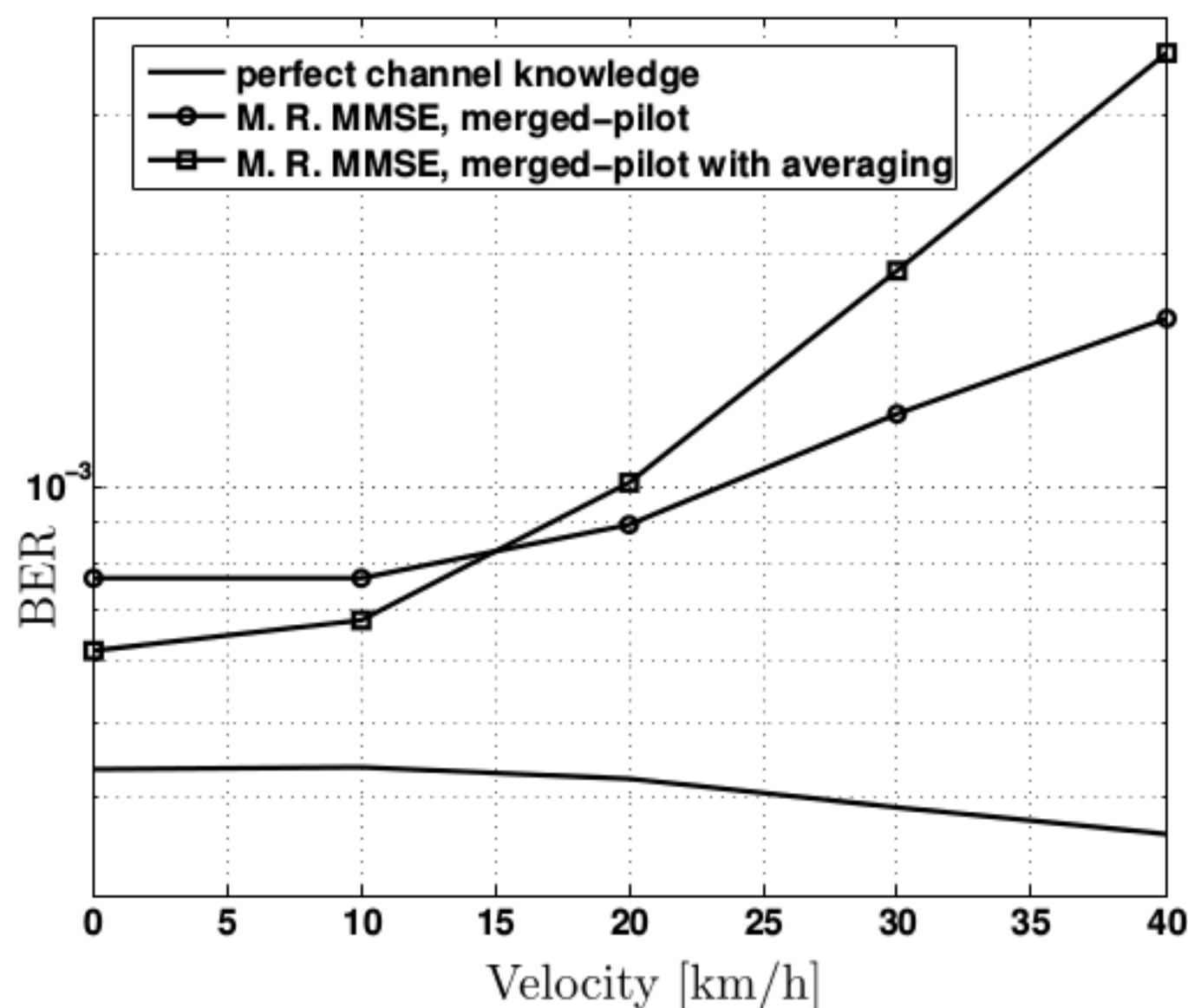
Fig. 5. LTE, coded BER. The simulations have been done for a 4 \times 4 MIMO system configured for spatial multiplexing using a ZF receiver for E_b/N_0 = 20dB .
