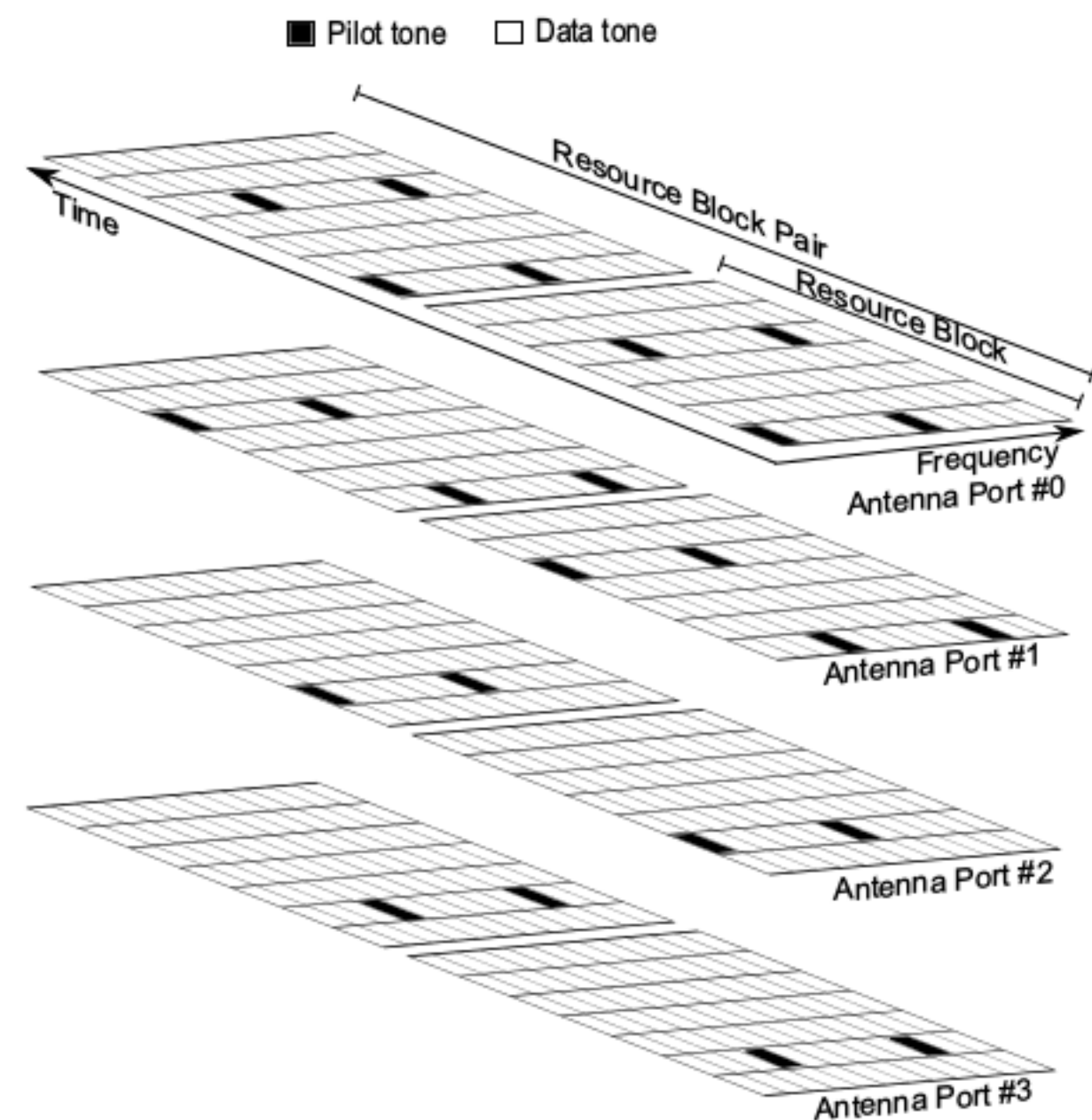
Fig. 1. LTE, scattered pilot structure for 4 \times 4 MIMO.
