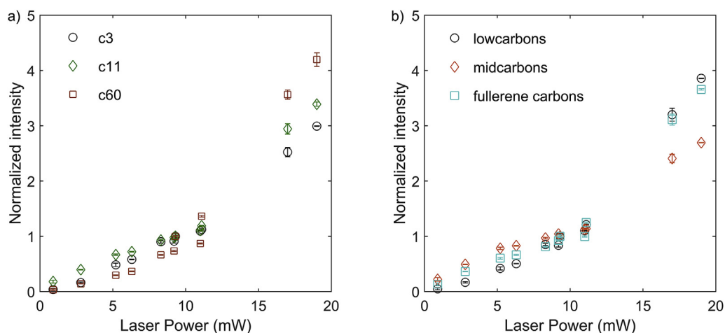
Fig. 3. SP-AMS laser intensity sweep on thermodenuded (250 °C) soot from mini-CAST OP6 and a) recorded C_3^+ , C_{11}^+ , and C_{60}^+ signals and b) recorded lowcarbon, midcarbon and fullerene carbon ion signals normalized to 9.3 mW laser power (i.e., signal is exactly 1 for 9.3 mW) and corrected for fluctuations in the miniCAST output concentration using equivalent BC (aethalometer). Laser power was recorded with an OPHIR laser power monitor from the bleed-through of the SP-AMS output coupler mirror. (A colour version of this figure can be viewed online.)
