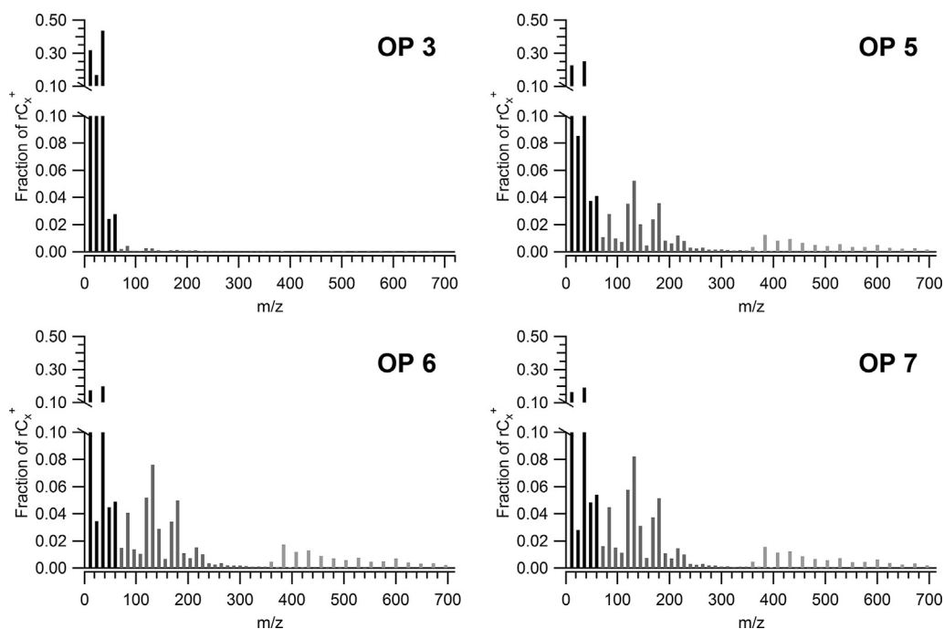
Fig. 2. SP-AMS normalized refractory carbon cluster ( rC_x^+ ) distributions for soot from miniCAST OP 3, 5, 6 and 7. Lowcarbons ( C_1^+-C_5^+ with m/z 12–60), midcarbons ( C_6^+-C_{29}^+ , m/z 72–348), fullerene carbons ( C_{30}^+-C_{59}^+ , m/z 360–708). Larger carbon clusters ( C_{\geq 6}^+ , m/z \geq 72 ) increased relative to lowcarbon clusters ( C_1^+-C_5^+ , m/z 12–60) with increasing OP.
