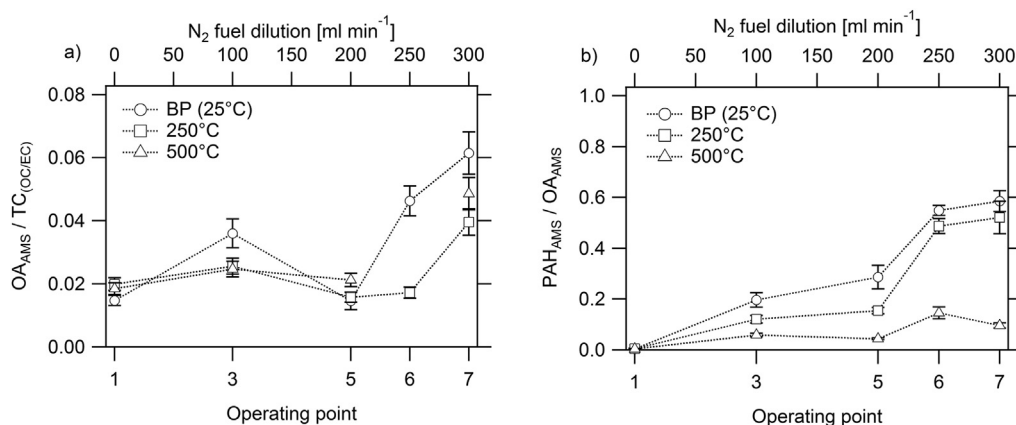
Fig. 4. a) Non-refractory organic aerosol (OA AMS , including PAHs) to total carbon mass (TC) ratios and b) polycyclic aromatic hydrocarbon (PAH AMS ) to OA AMS ratios for bypassing thermodenuder and furnace (BP), soot heated to 250 °C in a thermodenuder, and 500 °C in a ceramic furnace.
