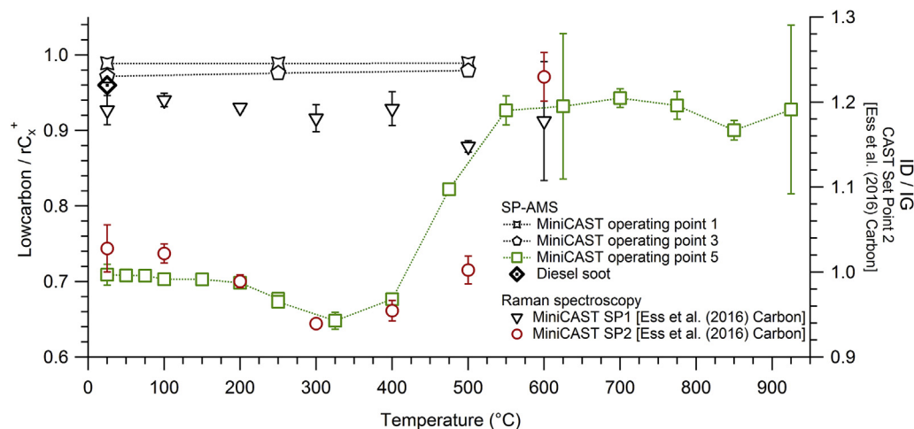
Fig. 10. Lowcarbon ( C_{\leq 5}^+ ) to rC_x^+ ratios (left axis) for: miniCAST OP5 soot during temperature ramping from 25 °C to 925 °C; miniCAST OP1 and OP3 soot at 25 °C, 250 °C, and 500 °C; diesel exhaust soot at 25 °C (untreated). The lowcarbon to rC_x^+ ratio is the complement to the large carbons ( C_{\geq 6}^+ ) to rC_x^+ ratio. Right axis, Raman spectroscopy analysis of the D and G band intensity ratios (ID/IG) of setpoint 1 and 2 (SP1 and SP2) soot from Ess et al. [79]. (A colour version of this figure can be viewed online.)
