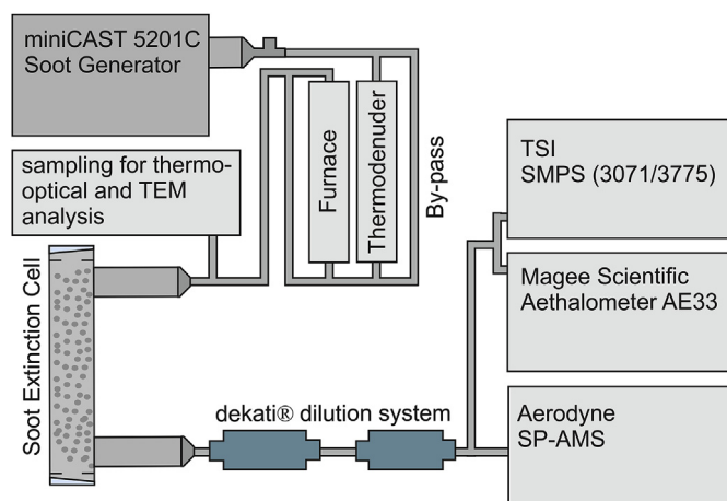
Fig. 1. Experimental set-up. The set-up included the soot extinction cell but is not part of the current analysis. Results on optical properties including the soot extinction cell have been published previously [35]. (A colour version of this figure can be viewed online.)
