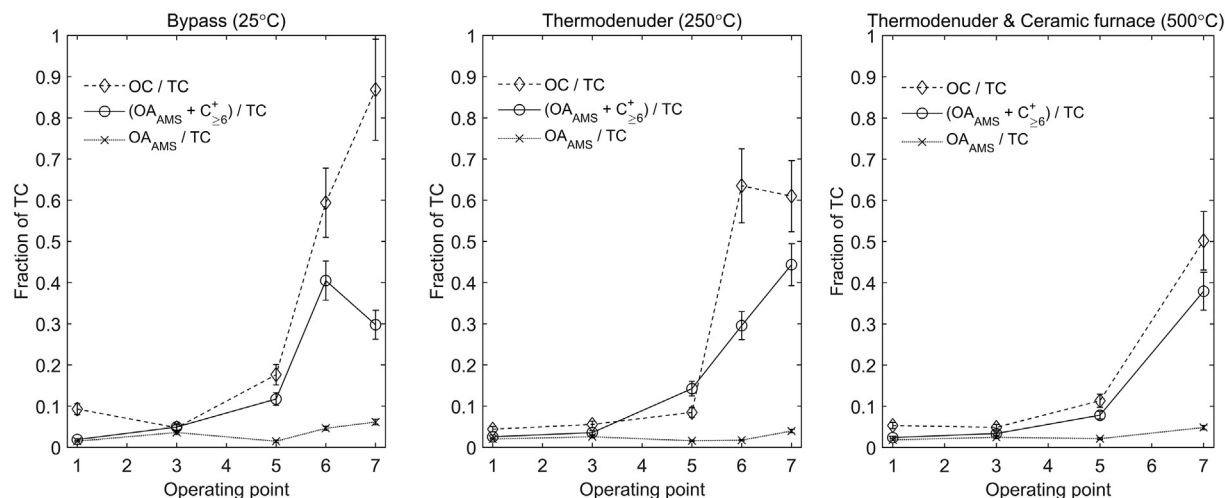
Fig. 6. OC (OC 1-4 + PC) to TC ratio, conventional AMS (SP-AMS laser off) OA AMS to TC ratio, and the sum of OA AMS and RIE RB equivalent large carbon (C >=6 + ) to TC ratio after no heating (25 °C), after heating to 250 °C in the thermodenuder, and after heating to 500 °C in the ceramic furnace. OP6 at 500 °C was not included due to a measurement error.
