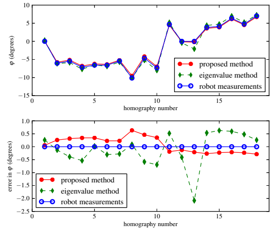
Figure 5: The upper plot shows the difference in orientation between consecutive images, and the lower plot shows the angular error. The plots show that our estimates of \varphi and the eigenvalue-based estimates of \varphi are both close to the truth (robot measurements).
