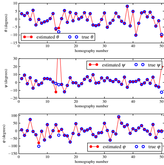
Figure 1: True and estimated values for \psi , \theta and \varphi for fifty randomly generated homographies. As can be seen, the estimation works well in most instances.
