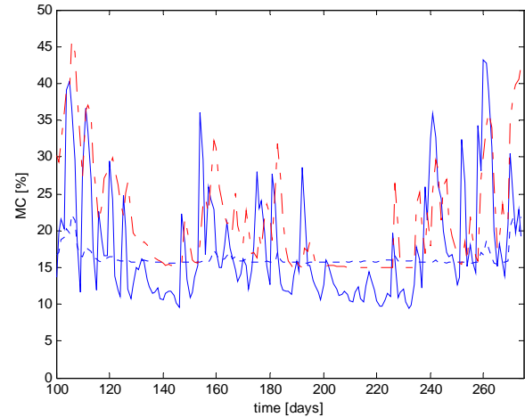
Figure 7: Comparison between modeled moisture content (solid line) and measured moisture content in a horizontal spruce board (dotted line) and a horizontal pine sapwood board (dashdot line) from day 100 (March 10 th ) to end of time period (August 31 st )
