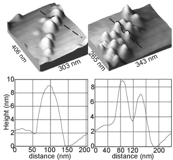
Fig. 2. 3D AFM images of dots at step-bunches on (a) GaInAs (b) \text{In}_{0.52}\text{Al}_{0.16}\text{Ga}_{0.32}\text{As} and corresponding surface line-scans. Line scans are indicated in (a) and (b).
