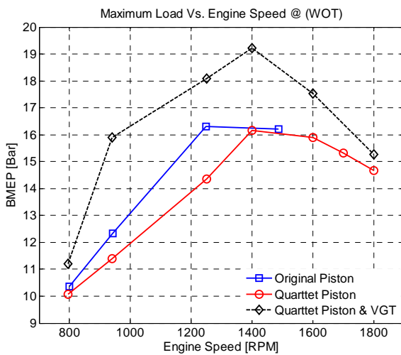
Figure 12: Maximum load after replacing the turbocharger to a VGT in compare with the other configurations
