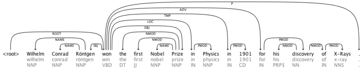
Figure 2: Dependency graph of the sentence Wilhelm Conrad Röntgen won the first Nobel Prize in Physics in 1901 for his discovery of X-Rays .
