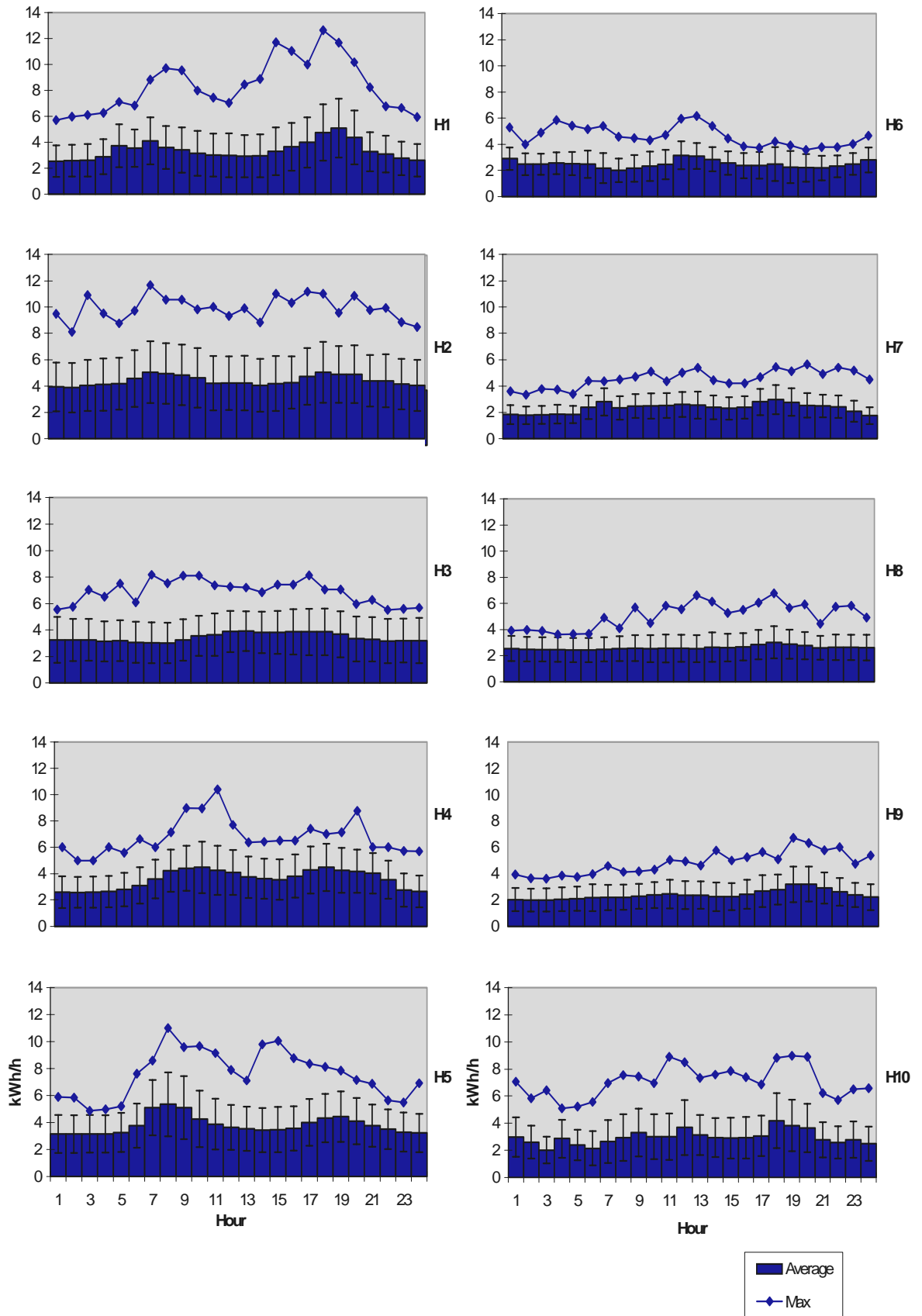
Figure 4.8. Daily load curve for winter season
