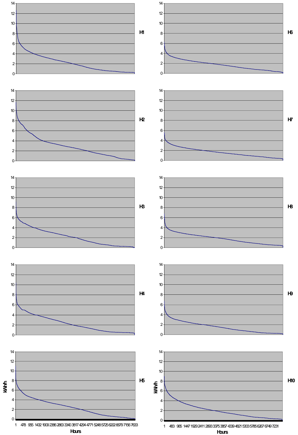
Figure 4.6. Load duration curve for 10 analyzed households
