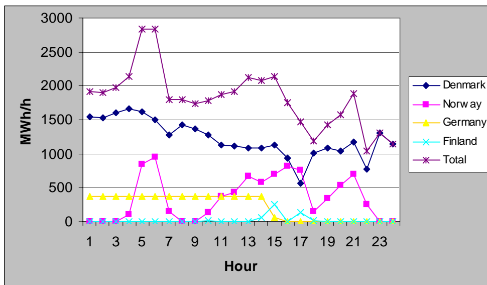
Figure 2.7. Import structure Feb.5, 2001 (Source: Svenska Kraftnät)
