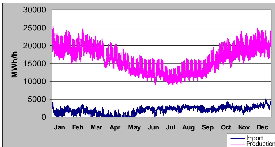
Figure 2.5. Hourly production and import to Sweden, 2002 (Source: Svenska Kraftnät)
