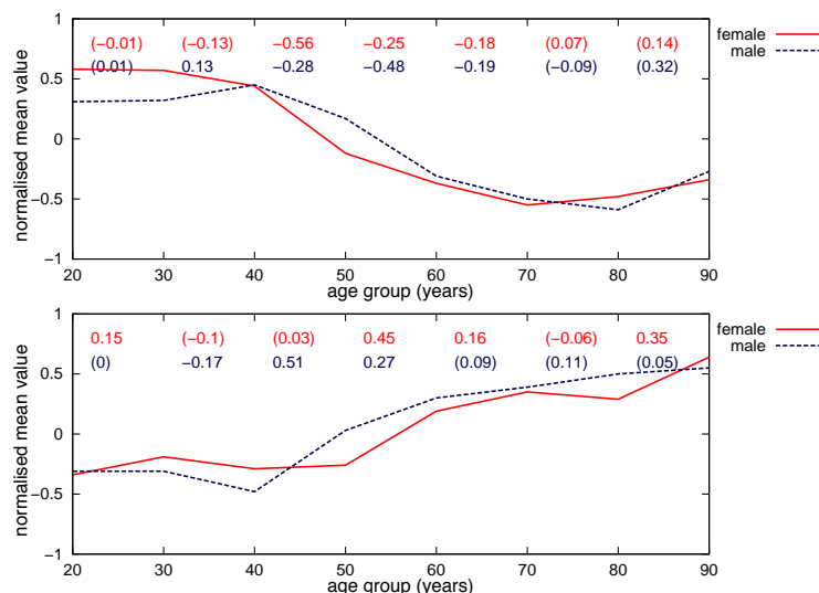
Fig. 11. Normalised (separately for each gender) tendencies for mean F_1 (top) and F_2 (bottom) ( [\varepsilon:] in the word själen ['\text{ʃ}\varepsilon:l\text{ə}n] )
