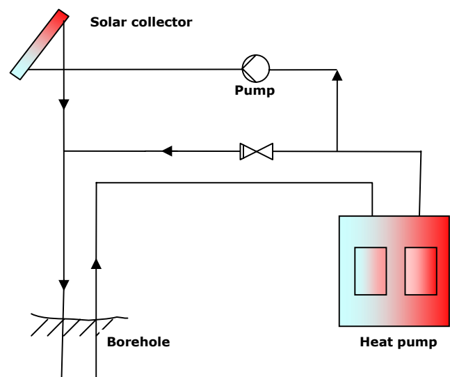
Fig. 4: Unglazed solar collector recharging the borehole.
