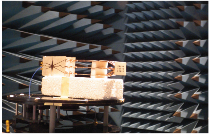
Fig. 3. Measurement setup in NSI anechoic chamber (photograph taken before covering the beamformer with absorbers).
