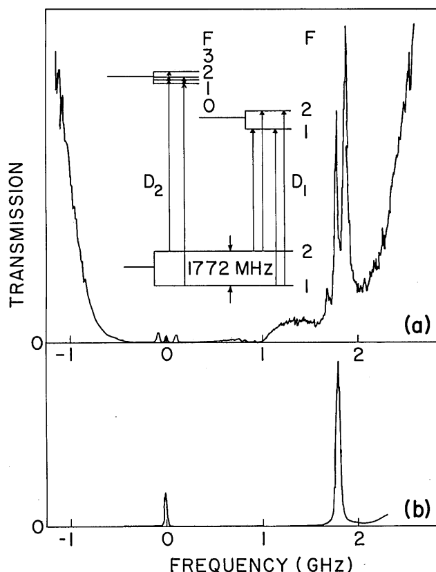
Fig. 2. Recordings for the sodium D lines and relevant transition hyperfine-structure diagrams. (a) D_1 line recording, using a 10-cm cell at 155°C. The probe-beam intensity is 8% of the pump beam intensity. (b) D_2 line recording, using a 30-cm cell at 141°C. The probe beam intensity is 0.5% of the pump beam intensity.
