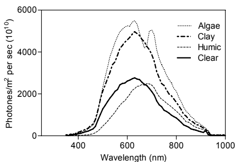
Figure 2. Spectral distribution of downwelling light in clear water and water with algae, clay and humic matter measured at 5.5 cm depth.
