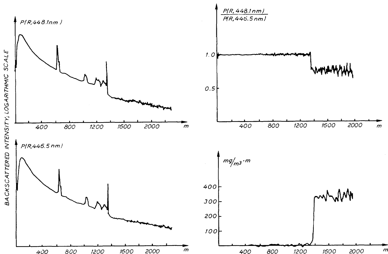
Fig. 6. Nitrogen dioxide DIAL measurement of a smokestack plume. Lidar is pointed just above the top of the smoke stack at a distance of 1350 m. Two lidar signals are shown to the left, and the DIAL curve is displayed at the upper right in the figure. Nitrogen dioxide is integrated across the plume and is shown as a step in the lower right curve.
