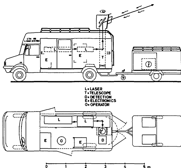
Fig. 2. Schematic of mobile laboratory.
