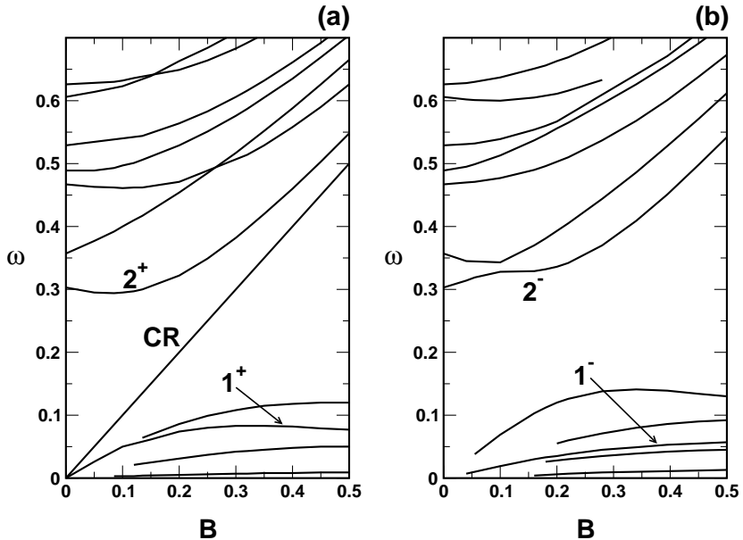
FIG. 2: The magnetic-field dispersions of the lowest-energy modes of the cyclotron [(panel (a))] and anti-cyclotron [(b)] polarization. Frequencies are measured in the units 9.12 \cdot 10^{12} \text{s}^{-1} , while the magnetic field strength unit equals 3.47 T. The label “CR” denotes the cyclotron resonance, “1” and “2” label the strongest modes whose oscillator strengths are depicted in a separate figure. The superscripts “+” and “-” refer, respectively, to the cyclotron and anti-cyclotron polarizations.
