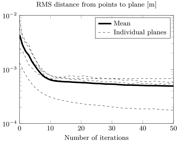
Fig. 6. Convergence results for experimental data gathered from 5 planes. The RMS distance between measurement points and the estimated planes are shown together with the mean over all planes.
