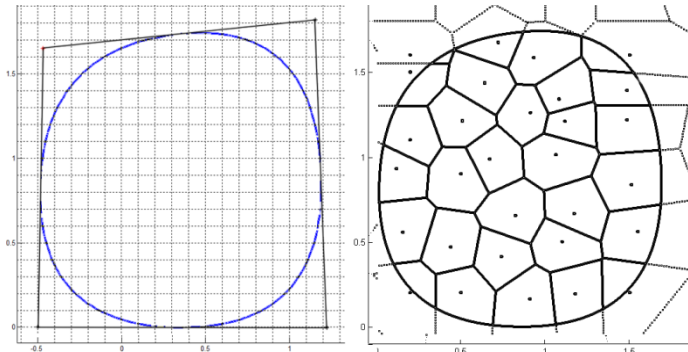
Figure 1. The interface through which the user of the GDS can define the table contour and review generated design candidates
