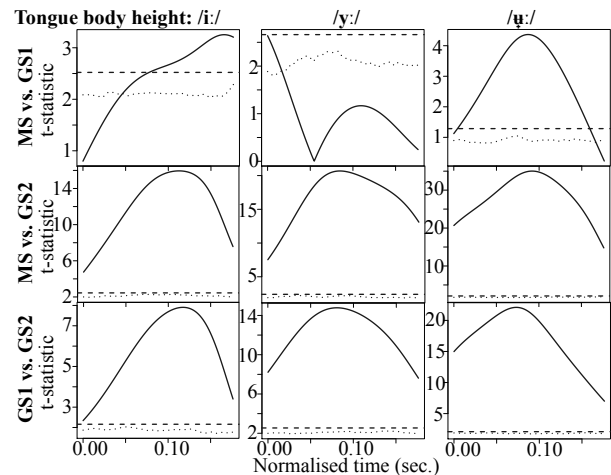
Figure 3: Pairwise functional t-tests for tongue body height of /i:/, /y:/, /ʉ:/ in Malmöhus Swedish (MS) and the two Gothenburg Swedish types (GS1 and GS2); solid lines: observed statistic, dashed lines: the permutation 0.05 critical value for the maximum of the t-statistic, dotted lines: the permutation critical value for the pointwise statistic.
