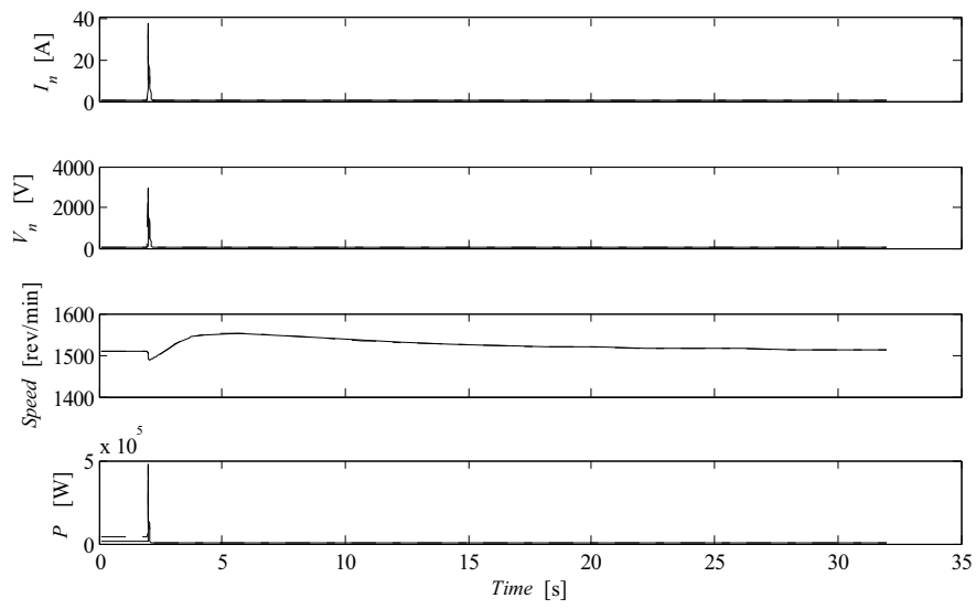
Figure A1.4.9 Phase A-B fault. Negative sequence current and voltage at fault point, generator speed, generator active power. l_{LI} = 2 km (solid lines) and l_{LI} = 6 km (dashed lines). P_{load} = 5 kW, R_f = 0 \Omega
