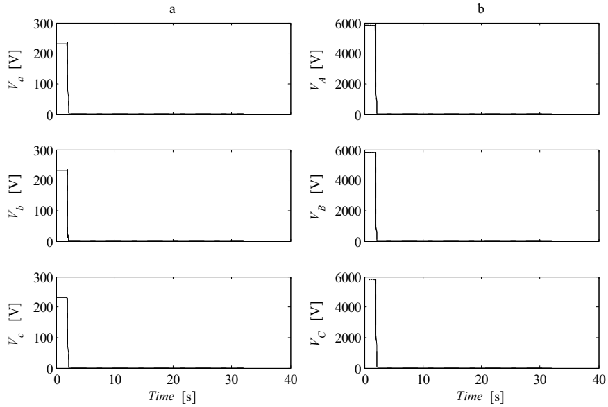
Figure A1.4.8 Phase A-B fault. a) Phase voltages at induction generator terminals b) Phase voltages on the high voltage side of step up transformer. l_{L1} = 2 \text{ km} (solid lines) and l_{L1} = 6 \text{ km} (dashed lines). P_{load} = 5 \text{ kW} , R_f = 0 \Omega
