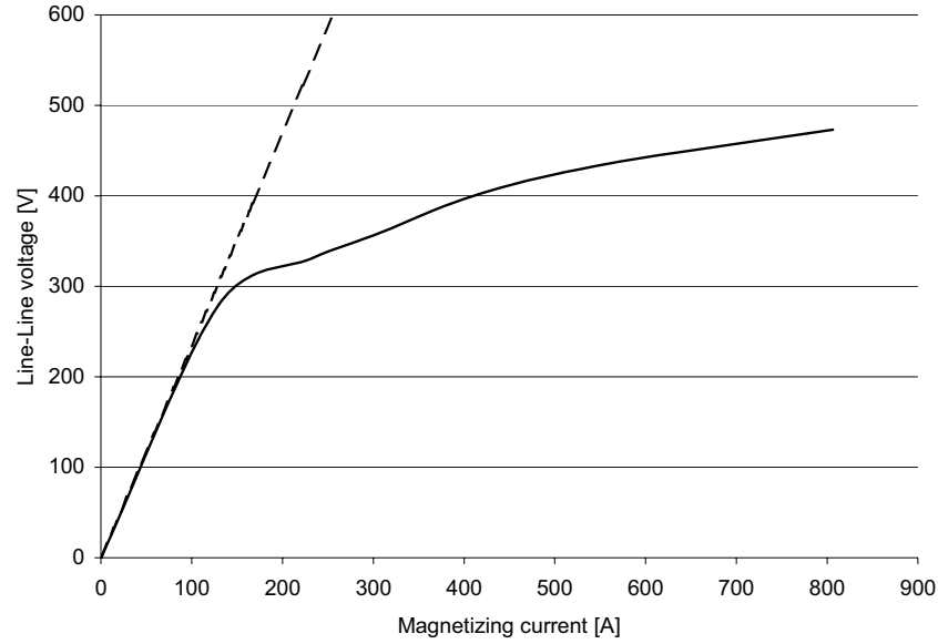
Figure 4.3 Main flux saturation curve for the induction generator
