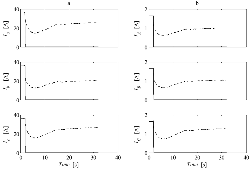
Figure A1.6.1 Phase a-b fault. a) Phase currents at induction generator terminals b) Phase currents on the high voltage side of step up transformer. R_f = 0 \, \Omega (solid lines) and R_f = 0.6 \, \Omega (dashed lines). l_{LI} = 4 \, \text{km} , P_{load} = 5 \, \text{kW}
