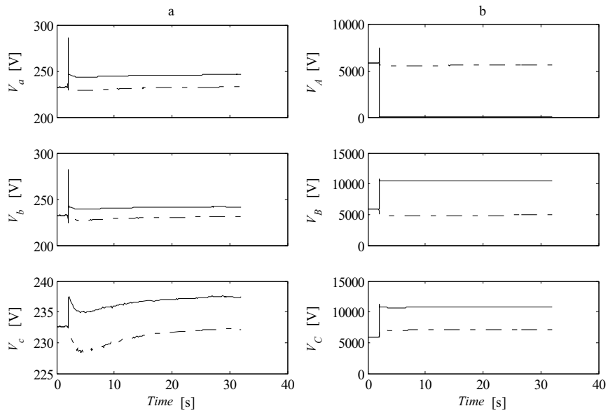
Figure A1.1.2 Phase A to earth fault. a) Phase voltages at induction generator terminals b) Phase voltages on the high voltage side of step up transformer. R_f = 0 \, \Omega (solid lines) and R_f = 5 \, k\Omega (dashed lines). l_{L1} = 4 \, km , P_{load} = 5 \, kW
