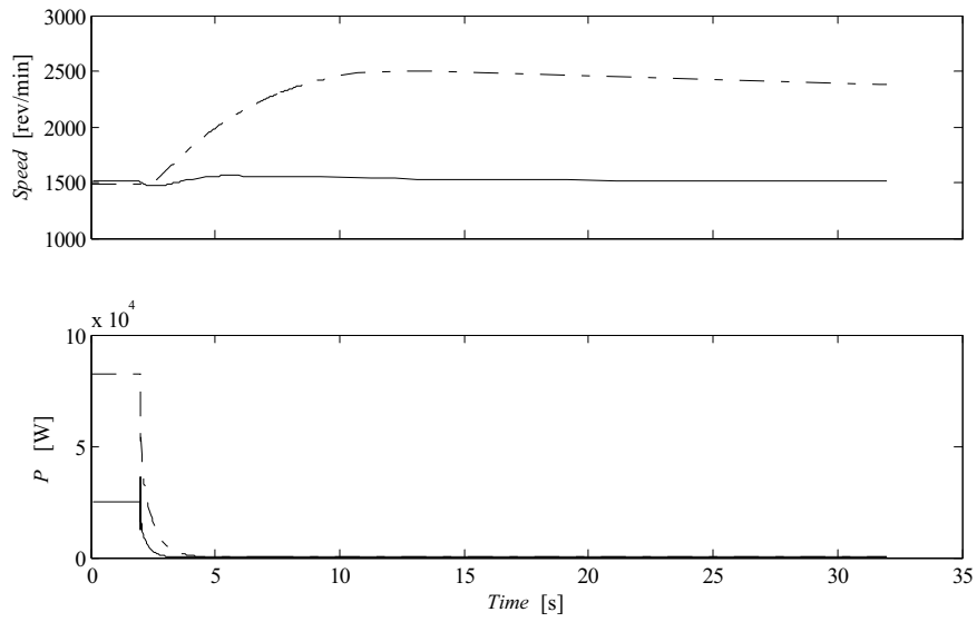
Figure A1.8.6 Three Phase fault. Generator speed, generator active power. P_{load} = 5 kW (solid lines) and P_{load} = 85 kW (dashed lines). l_{L1} = 4 km, R_f = 0 \Omega
