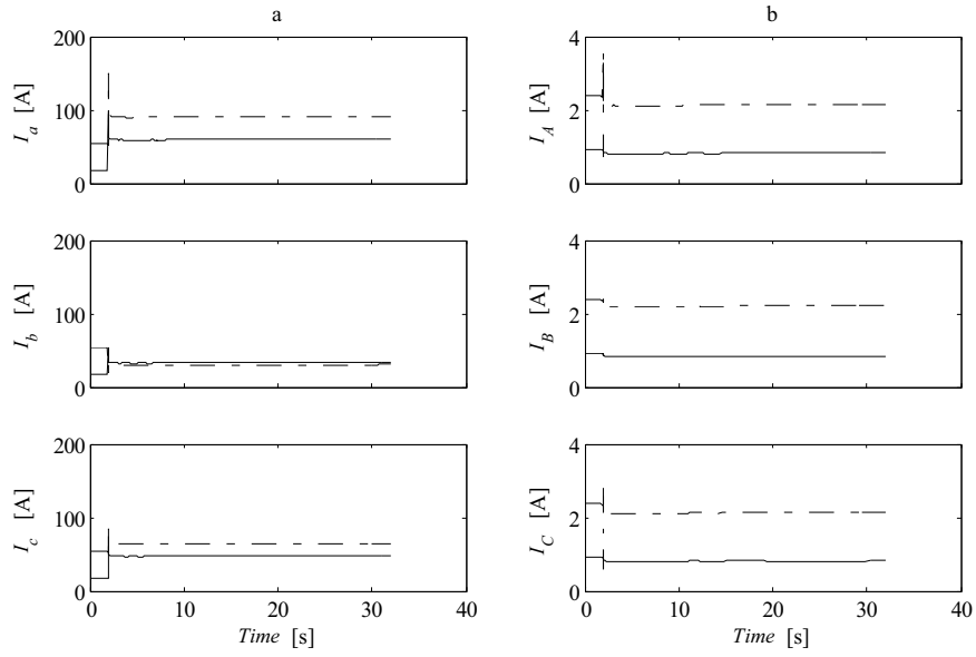
Figure A1.2.7 Phase a to earth fault. a) Phase currents at induction generator terminals b) Phase currents on the high voltage side of step up transformer. l_{LI} = 2 km (solid lines) and l_{LI} = 6 km (dashed lines). P_{load} = 5 kW, R_f = 0 \Omega
