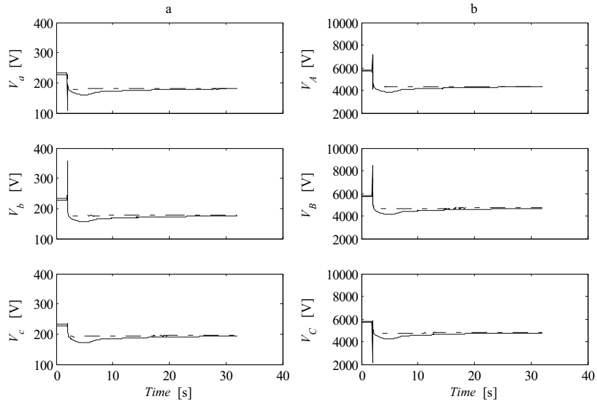
Figure A1.5.5 Phase a-b fault. a) Phase voltages at induction generator terminals b) Phase voltages on the high voltage side of step up transformer. P_{load} = 5 \text{ kW} (solid lines) and P_{load} = 85 \text{ kW} (dashed lines). l_{L1} = 4 \text{ km} , R_f = 0 \Omega
