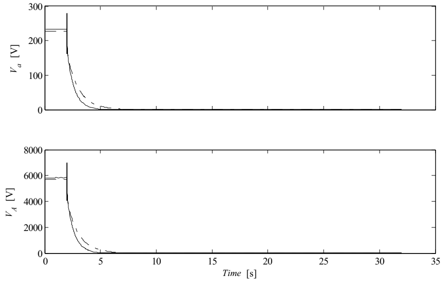
Figure A1.8.5 Three Phase fault. a) Phase voltage at induction generator terminals b) Phase voltage on the high voltage side of step up transformer. P_{load} = 5 kW (solid lines) and P_{load} = 85 kW (dashed lines). l_{L1} = 4 km, R_f = 0 \Omega
