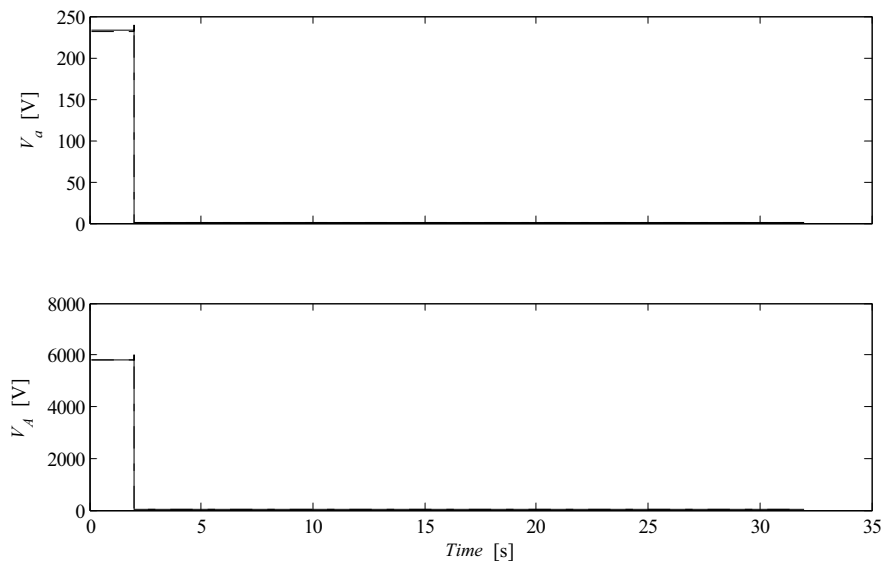
Figure A1.9.8 Three Phase fault. a) Phase voltage at induction generator terminals b) Phase voltage on the high voltage side of step up transformer. l_{L1} = 2 \text{ km} (solid lines) and l_{L1} = 6 \text{ km} (dashed lines). P_{load} = 5 \text{ kW} , R_f = 0 \Omega
