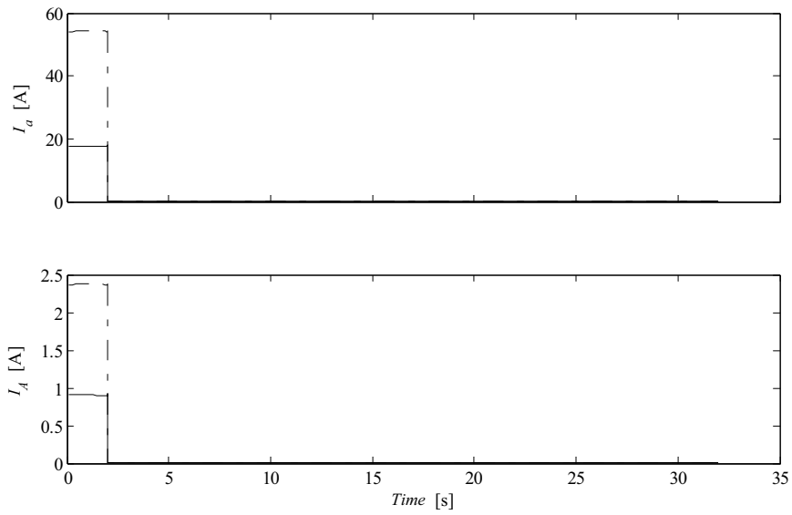
Figure A1.9.7 Three Phase fault. a) Phase current at induction generator terminals b) Phase current on the high voltage side of step up transformer. l_{L1} = 2 \text{ km} (solid lines) and l_{L1} = 6 \text{ km} (dashed lines). P_{load} = 5 \text{ kW} , R_f = 0 \Omega
