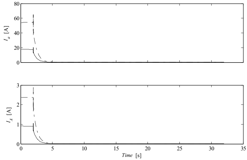
Figure A1.8.7 Three Phase fault. a) Phase current at induction generator terminals b) Phase current on the high voltage side of step up transformer. l_{L1} = 2 \text{ km} (solid lines) and l_{L1} = 6 \text{ km} (dashed lines). P_{load} = 5 \text{ kW} , R_f = 0 \text{ } \Omega
