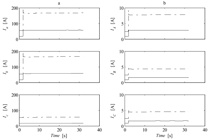
Figure A1.1.7 Phase A to earth fault. a) Phase currents at induction generator terminals b) Phase currents on the high voltage side of step up transformer. l_{LI} = 2 \text{ km} (solid lines) and l_{LI} = 6 \text{ km} (dashed lines). P_{load} = 5 \text{ kW} , R_f = 0 \Omega
