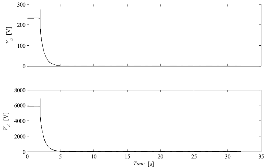
Figure A1.8.8 Three Phase fault. a) Phase voltage at induction generator terminals b) Phase voltage on the high voltage side of step up transformer. l_{L1} = 2 \text{ km} (solid lines) and l_{L1} = 6 \text{ km} (dashed lines). P_{load} = 5 \text{ kW} , R_f = 0 \text{ } \Omega
