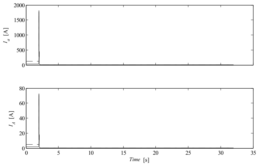
Figure A1.7.4 Three Phase fault. a) Phase current at induction generator terminals b) Phase current on the high voltage side of step up transformer. P_{load} = 5 kW (solid lines) and P_{load} = 85 kW (dashed lines). l_{L1} = 4 km, R_f = 0 \Omega
