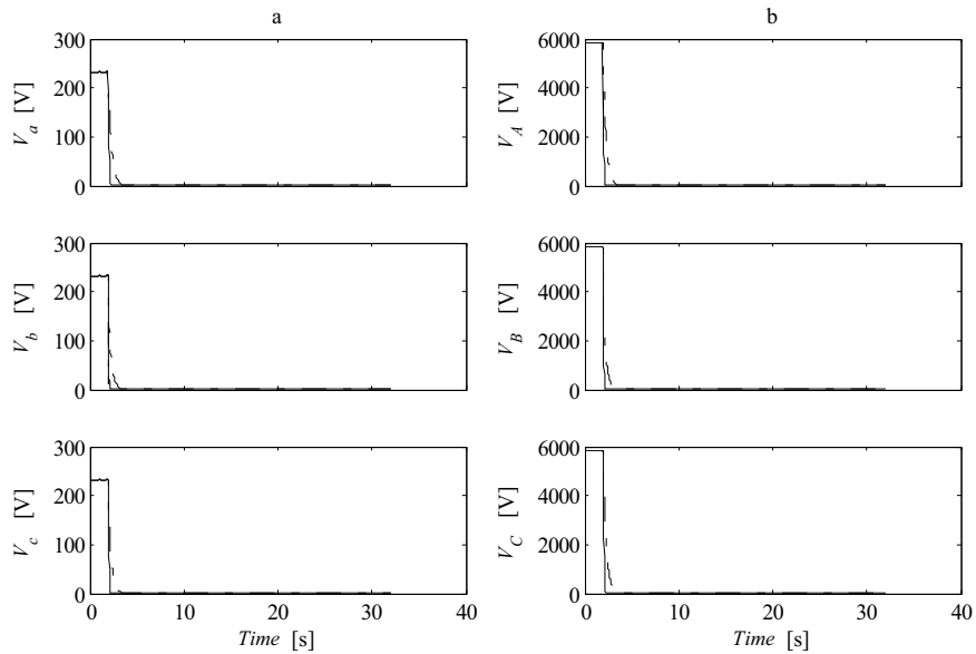
Figure A1.4.2 Phase A-B fault. a) Phase voltages at induction generator terminals b) Phase voltages on the high voltage side of step up transformer. R_f = 0 \, \Omega (solid lines) and R_f = 200 \, \Omega (dashed lines). l_{L1} = 4 \, \text{km} , P_{load} = 5 \, \text{kW}
