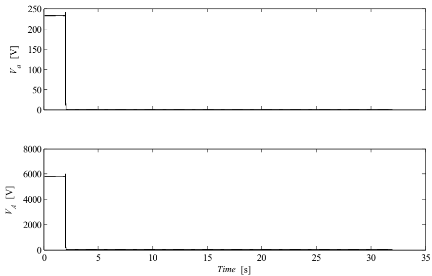
Figure A1.7.8 Three Phase fault. a) Phase voltage s at induction generator terminals b) Phase voltage on the high voltage side of step up transformer. l_{L1} = 2 \text{ km} (solid lines) and l_{L1} = 6 \text{ km} (dashed lines). P_{load} = 5 \text{ kW} , R_f = 0 \text{ } \Omega
