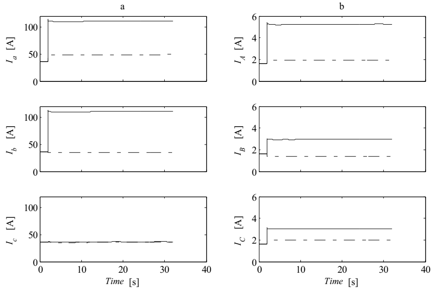
Figure A1.1.1 Phase A to earth fault. a) Phase currents at induction generator terminals b) Phase currents on the high voltage side of step up transformer. R_f = 0 \, \Omega (solid lines) and R_f = 5 \, k\Omega (dashed lines). l_{L1} = 4 \, km , P_{load} = 5 \, kW
