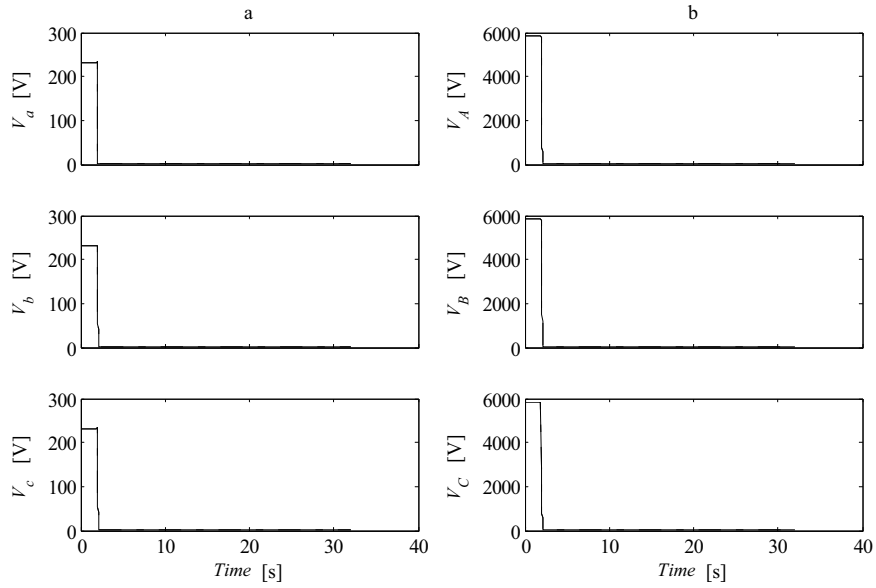
Figure A1.3.8 Phase a to earth fault. a) Phase voltages at induction generator terminals b) Phase voltages on the high voltage side of step up transformer. l_{LI} = 2 km (solid lines) and l_{LI} = 6 km (dashed lines). P_{load} = 5 kW, R_f = 0 \Omega
