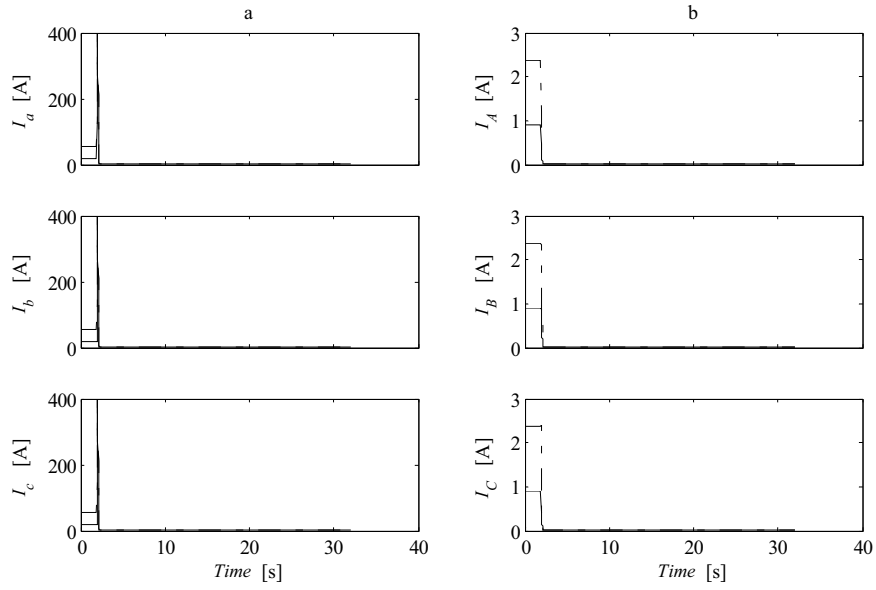
Figure A1.3.7 Phase a to earth fault. a) Phase currents at induction generator terminals b) Phase currents on the high voltage side of step up transformer. l_{LI} = 2 km (solid lines) and l_{LI} = 6 km (dashed lines). P_{load} = 5 kW, R_f = 0 \Omega
