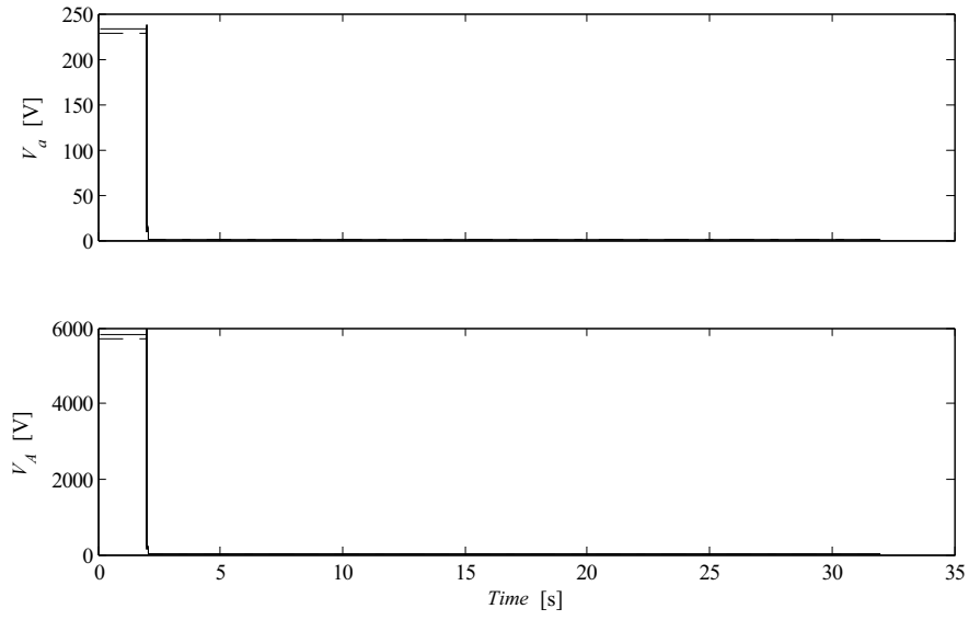
Figure A1.7.5 Three Phase fault. a) Phase voltage at induction generator terminals b) Phase voltage on the high voltage side of step up transformer. P_{load} = 5 kW (solid lines) and P_{load} = 85 kW (dashed lines). l_{L1} = 4 km, R_f = 0 \Omega
