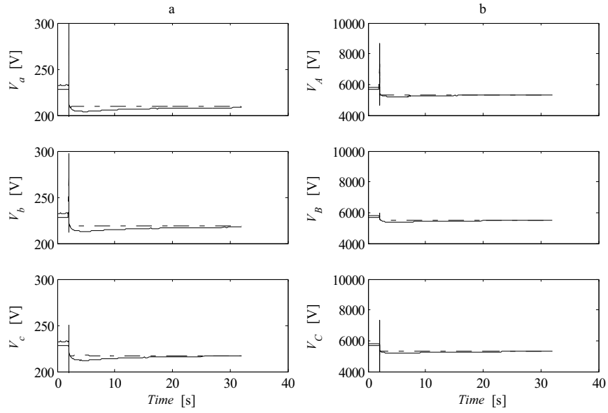
Figure A1.2.5 Phase a to earth fault. a) Phase voltages at induction generator terminals b) Phase voltages on the high voltage side of step up transformer. P_{load} = 5 \text{ kW} (solid lines) and P_{load} = 85 \text{ kW} (dashed lines). l_{L1} = 4 \text{ km} , R_f = 0 \Omega
