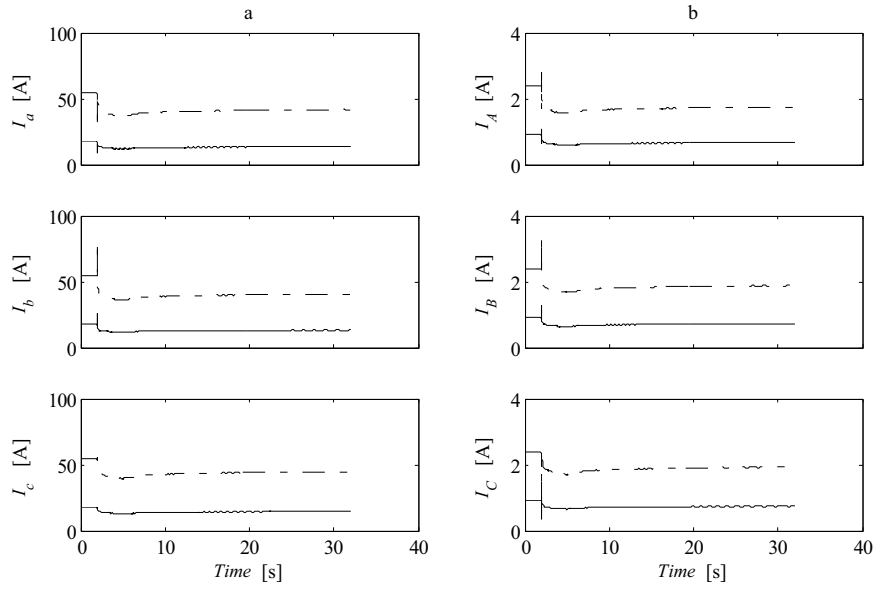
Figure A1.5.7 Phase a-b fault. a) Phase currents at induction generator terminals b) Phase currents on the high voltage side of step up transformer. l_{LI} = 2 km (solid lines) and l_{LI} = 6 km (dashed lines). P_{load} = 5 kW, R_f = 0 \Omega
