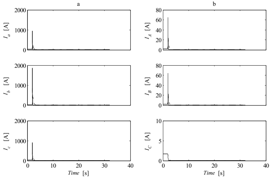
Figure A1.4.1 Phase A-B fault. a) Phase currents at induction generator terminals b) Phase currents on the high voltage side of step up transformer. R_f = 0 \, \Omega (solid lines) and R_f = 200 \, \Omega (dashed lines). l_{L1} = 4 \, \text{km} , P_{load} = 5 \, \text{kW}
