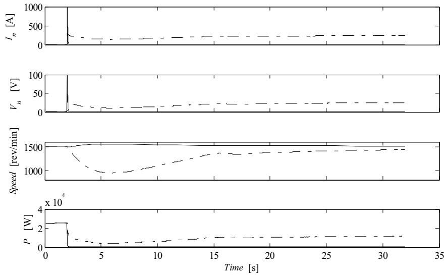
Figure A1.6.3 Phase a-b fault. Negative sequence current and voltage at fault point, generator speed, generator active power. R_f = 0 \, \Omega (solid lines) and R_f = 0.6 \, \Omega (dashed lines). l_{L1} = 4 \, \text{km} , P_{load} = 5 \, \text{kW}
