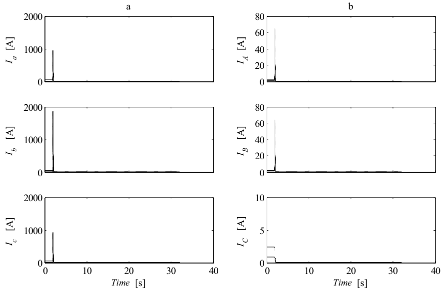
Figure A1.4.7 Phase A-B fault. a) Phase currents at induction generator terminals b) Phase currents on the high voltage side of step up transformer. l_{L1} = 2 \text{ km} (solid lines) and l_{L1} = 6 \text{ km} (dashed lines). P_{load} = 5 \text{ kW} , R_f = 0 \Omega
