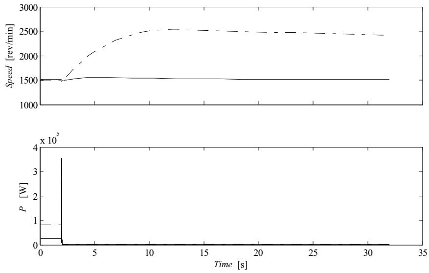
Figure A1.7.6 Three Phase fault. Generator speed, generator active power. P_{load} = 5 kW (solid lines) and P_{load} = 85 kW (dashed lines). l_{L1} = 4 km, R_f = 0 \Omega
