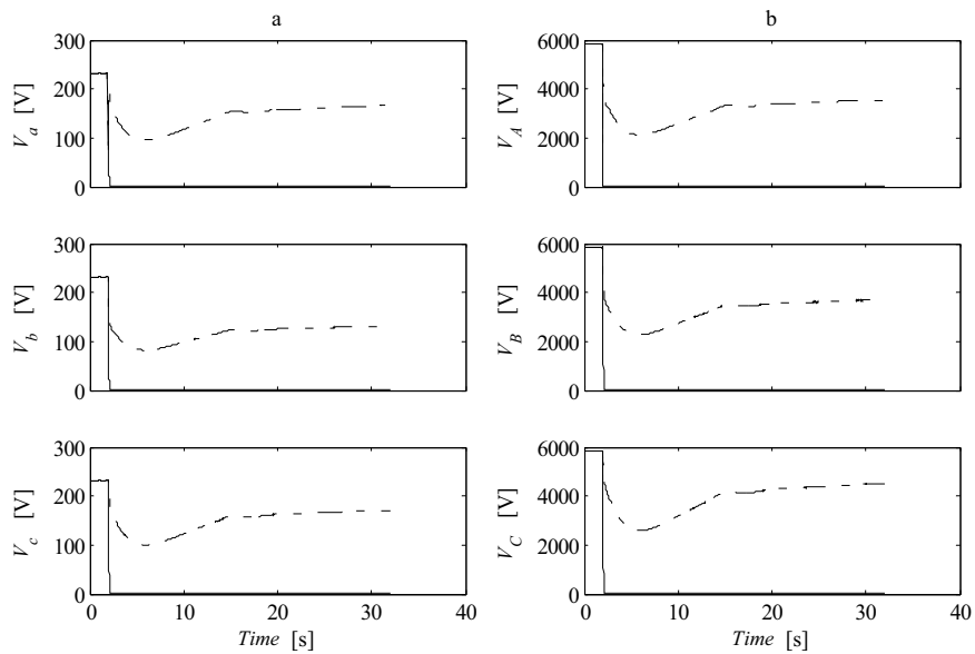
Figure A1.6.2 Phase a-b fault. a) Phase voltages at induction generator terminals b) Phase voltages on the high voltage side of step up transformer. R_f = 0 \, \Omega (solid lines) and R_f = 0.6 \, \Omega (dashed lines). l_{LI} = 4 \, \text{km} , P_{load} = 5 \, \text{kW}
