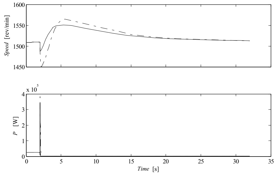
Figure A1.7.3 Three Phase fault. Generator speed, generator active power. R_f = 0 \Omega (solid lines) and R_f = 200 \Omega (dashed lines). l_{L1} = 4 km, P_{load} = 5 kW
