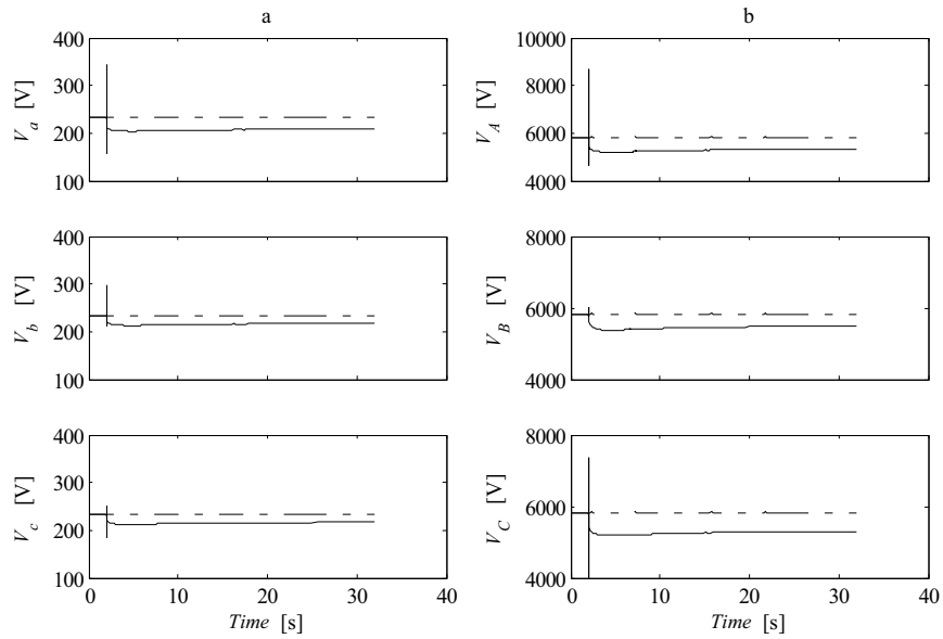
Figure A1.2.2 Phase a to earth fault. a) Phase voltages at induction generator terminals b) Phase voltages on the high voltage side of step up transformer. R_f = 0 \Omega (solid lines) and R_f = 5 k\Omega (dashed lines). l_{L1} = 4 km , P_{load} = 5 kW
