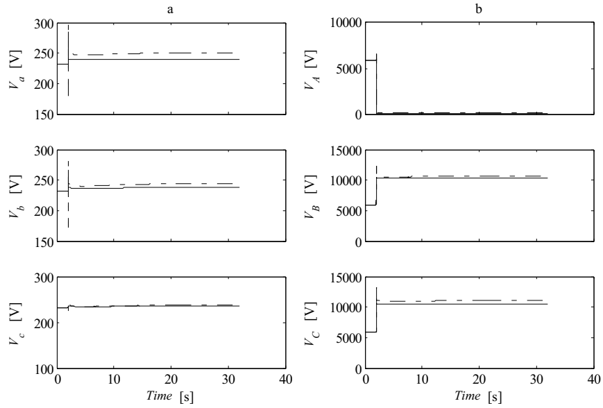
Figure A1.1.8 Phase A to earth fault. a) Phase voltages at induction generator terminals b) Phase voltages on the high voltage side of step up transformer. l_{LI} = 2 \text{ km} (solid lines) and l_{LI} = 6 \text{ km} (dashed lines). P_{load} = 5 \text{ kW} , R_f = 0 \Omega
