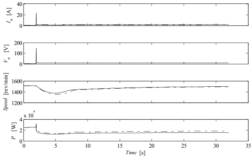
Figure A1.5.3 Phase a-b fault. Negative sequence current and voltage at fault point, generator speed, generator active power. R_f = 0 \, \Omega (solid lines) and R_f = 0.6 \, \Omega (dashed lines). l_{L1} = 4 \, \text{km} , P_{load} = 5 \, \text{kW}
