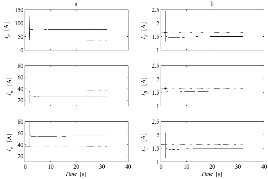
Figure A1.2.1 Phase a to earth fault. a) Phase currents at induction generator terminals b) Phase currents on the high voltage side of step up transformer. R_f = 0 \Omega (solid lines) and R_f = 5 k\Omega (dashed lines). l_{L1} = 4 km , P_{load} = 5 kW
