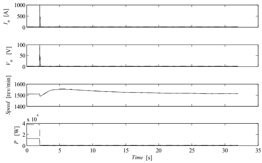
Figure A1.6.9 Phase a-b fault. Negative sequence current and voltage at fault point, generator speed, generator active power. l_{LI} = 2 km (solid lines) and l_{LI} = 6 km (dashed lines). P_{load} = 5 kW, R_f = 0 \Omega
