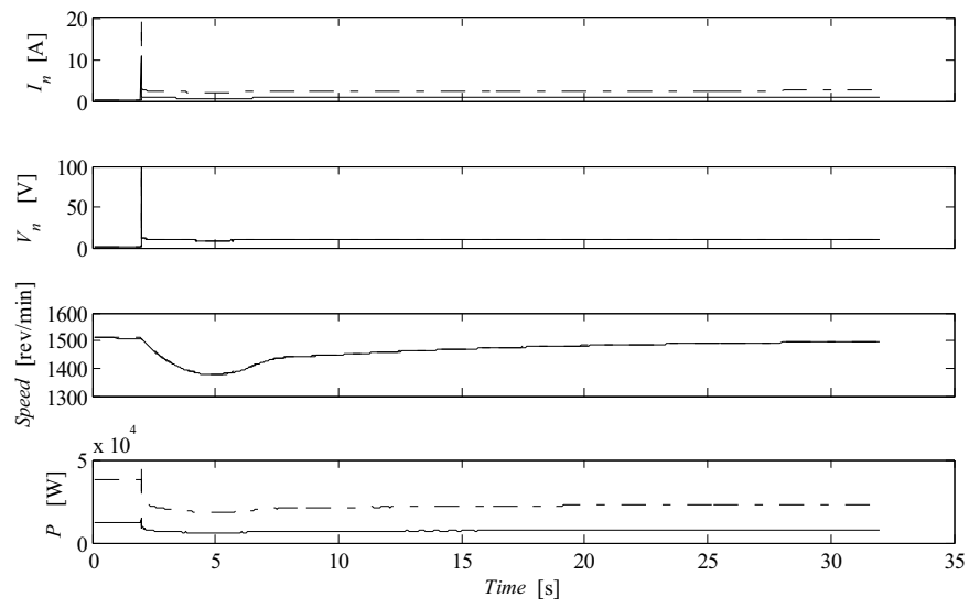
Figure A1.5.9 Phase a-b fault. Negative sequence current and voltage at fault point, generator speed, generator active power. l_{LI} = 2 km (solid lines) and l_{LI} = 6 km (dashed lines). P_{load} = 5 kW, R_f = 0 \Omega
