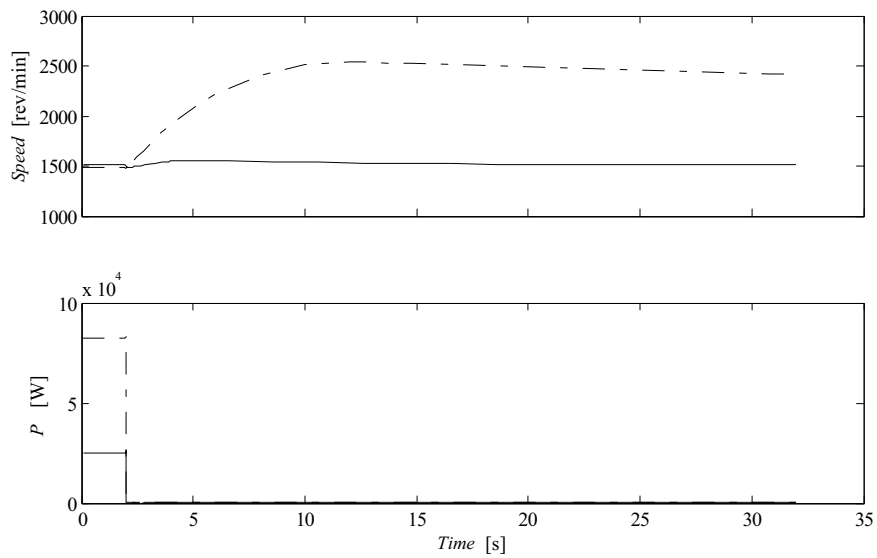
Figure A1.9.6 Three Phase fault. Generator speed, generator active power. P_{load} = 5 \text{ kW} (solid lines) and P_{load} = 85 \text{ kW} (dashed lines). L_{LI} = 4 \text{ km} , R_f = 0 \Omega
