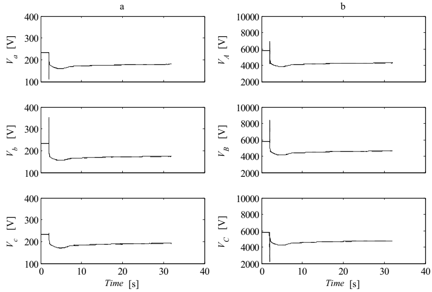
Figure A1.5.8 Phase a-b fault. a) Phase voltages at induction generator terminals b) Phase voltages on the high voltage side of step up transformer. l_{LI} = 2 km (solid lines) and l_{LI} = 6 km (dashed lines). P_{load} = 5 kW, R_f = 0 \Omega
