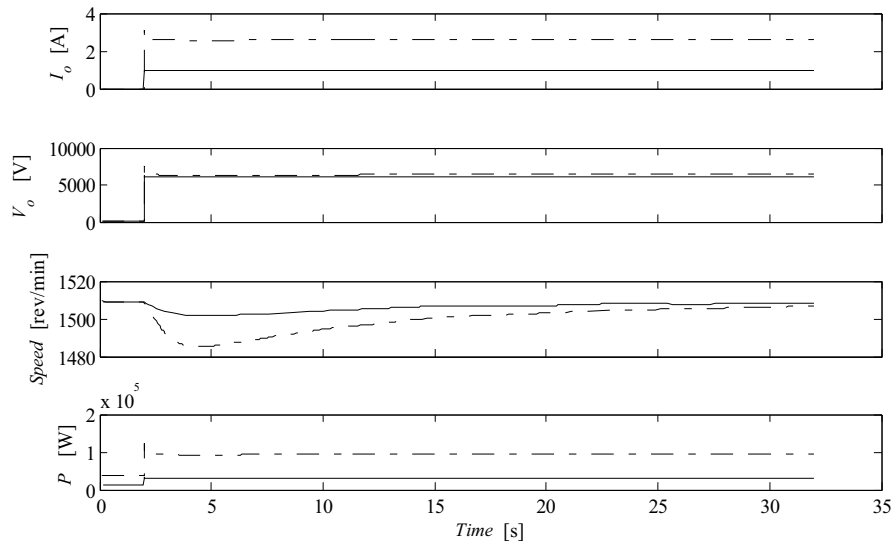
Figure A1.1.9 Phase A to earth fault. Zero sequence current and voltage at fault point, generator speed, generator active power. l_{LI} = 2 km (solid lines) and l_{LI} = 6 km (dashed lines). P_{load} = 5 kW, R_f = 0 \Omega
