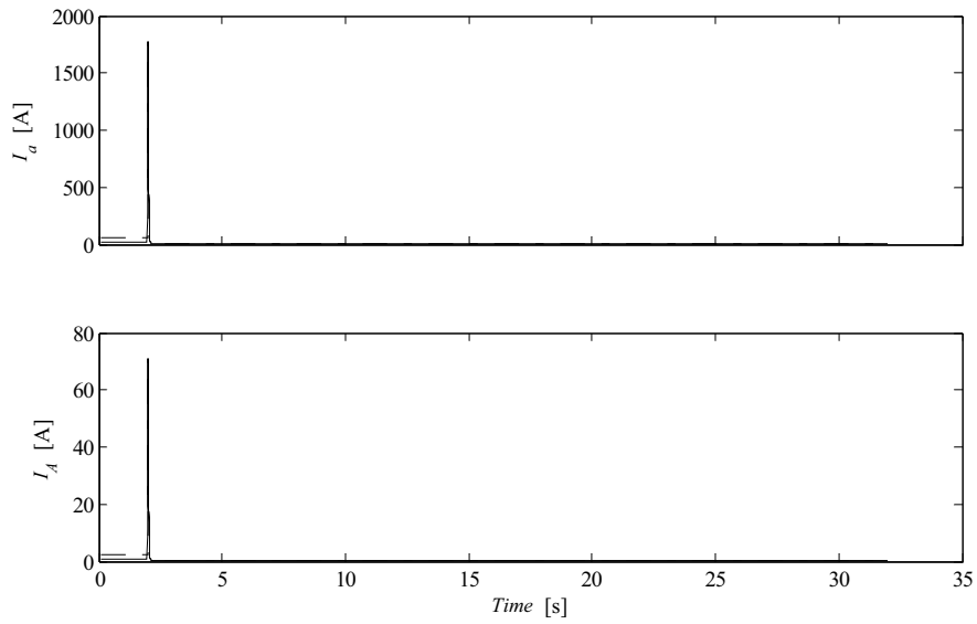
Figure A1.7.7 Three Phase fault. a) Phase current at induction generator terminals b) Phase current on the high voltage side of step up transformer. l_{L1} = 2 \text{ km} (solid lines) and l_{L1} = 6 \text{ km} (dashed lines). P_{load} = 5 \text{ kW} , R_f = 0 \text{ } \Omega
