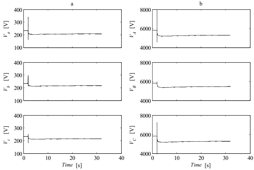
Figure A1.2.8 Phase a to earth fault. a) Phase voltages at induction generator terminals b) Phase voltages on the high voltage side of step up transformer. l_{LI} = 2 km (solid lines) and l_{LI} = 6 km (dashed lines). P_{load} = 5 kW, R_f = 0 \Omega
