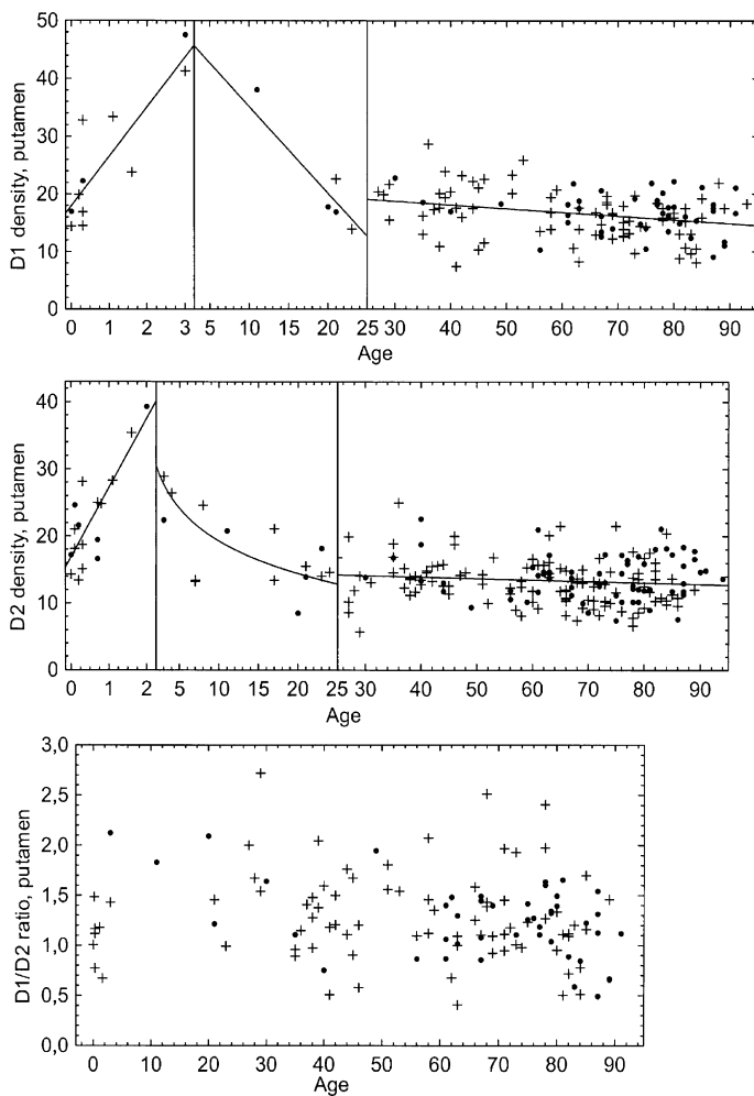
Fig. 2. Density of D1- and D2-receptors in the putamen, and D1/D2 ratio, based on postmortem data published by Seeman et al. (1987), from 244 cases in the general population. The sign ● marks females and + marks males. The regression lines are calculated for the rise, decline, and adult periods. The correlation between receptor density and age during the rise period was 0.86 for D1-receptors and 0.82 for D2-receptors. Note that for some individuals only D1- or D2-receptor density was measured, resulting in a lower number of individuals in the D1/D2 ratio plot. (In 24 of the cases the densities in the putamen were not measured, instead the figures were estimated from the available values for the caudate nucleus. The correlation between receptor density in the putamen and caudate nucleus was 0.82 in this study.)
