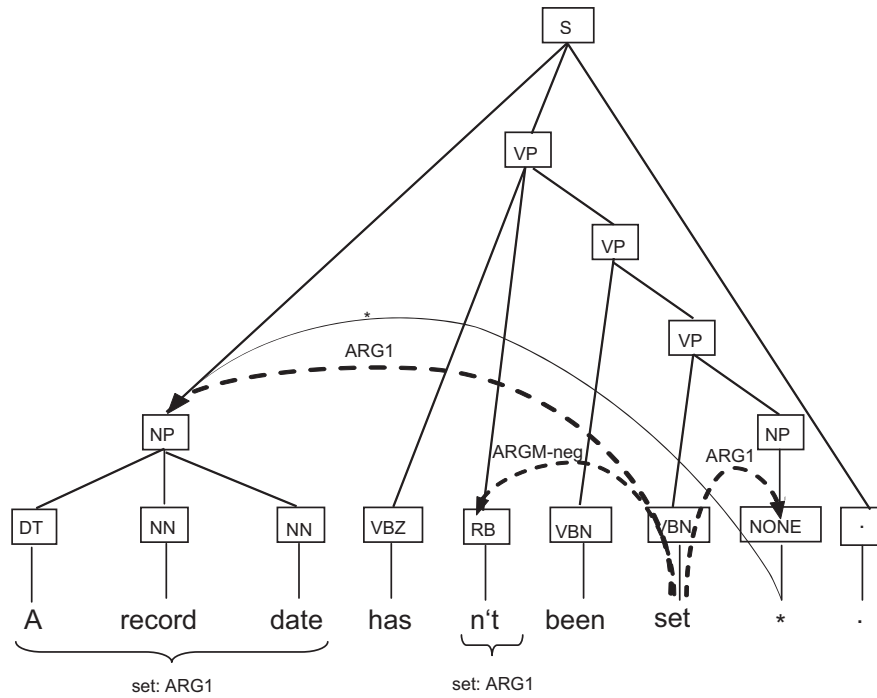
Figure 2: The phrase structure representation of sentence wsj02wsj_0202 in PropBank
