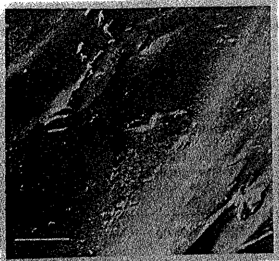
Fig 11. Replica surface of quartz flake used to scrape fresh elk bone for 15 minutes. a) before and b) after etching in \text{NH}_4\text{HF}_2 for 10 minutes. From Knutsson 1988b, fig 83.
