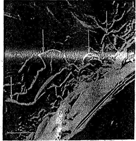
Fig 4. SEM photograph of replica surface of mechanically ruptured edges on a quartz flake. Scale: 70 my. From Knutsson 1988a, fig 67.
