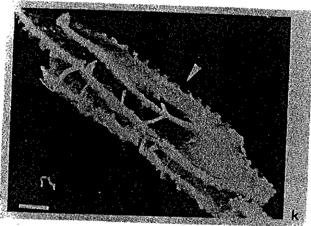
Fig 5 SEM micrographs of residues. k) Plant residue (Gramineae family) on the edge of a Middle Bronze Age flint "sickle" from Denmark. l) Reference specimen of a stem fragment of a Gramineae. Scale = 10 microns. From Anderson-Gerfaud 1986, Plate 19.
