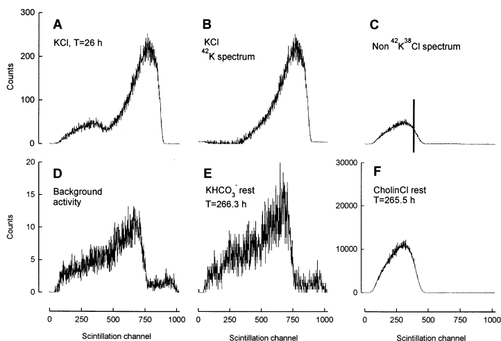
Figure 3. Deduction of a decay spectrum for non- ^{42}\text{K}:^{38}\text{Cl} isotopes, and illustration of 'rest' and background decay spectra. The non- ^{42}\text{K}:^{38}\text{Cl} spectrum was obtained as follows: C = A - B [A representing conditions after the complete disappearance of ^{38}\text{Cl} (same as D in Fig. 3) and B representing the specific ^{42}\text{K} spectrum (same as F in Fig. 3)]. The non- ^{42}\text{K}:^{38}\text{Cl} spectrum is qualitatively indistinguishable from the \text{CholineCl} rest spectrum, F, obtained after the complete disappearance of ^{38}\text{Cl} and, because thereof, indicative of the samples containing no unaccountable contamination. E, \text{HCO}_3 rest spectrum after complete disappearance of ^{42}\text{K} . Statistically, this rest spectrum does not differ from the background decay spectrum (D) and, because hereof, indicative that no unaccountable contaminations are present in the material. The vertical bar in C delimits the scintillation channels 1–380 whose signals were excluded from further data evaluation, since they were adding to noise more than to relevant information.
