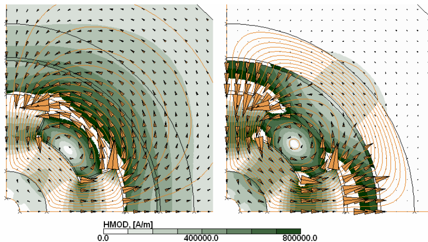
Figure 2.9: Magnetizing field of the magnetizer. The magnetizer consists of a slotted core where angular width is changed. The magnet-ring is placed on top of magnetizer and can be with solid iron yoke (right) or without it (left).
