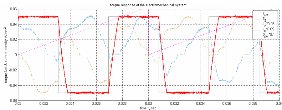
Figure 6.16: Torque response of the electromechanical system at the square wave reference of \pm 50 Nmm and 130 Hz.
