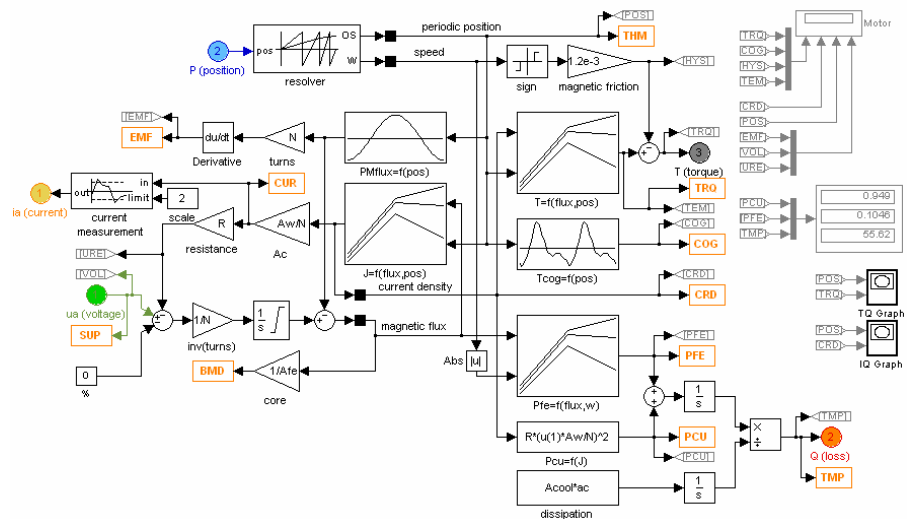
Figure 6.6: The model for electromechanical energy conversion.
