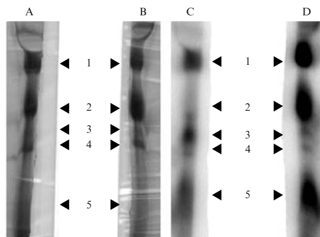
Figure 1: Coomassie stain and Phosphorimage of ^{32}P -labeled protein complexes from a blue native gel of redox treated chloroplasts. (A) and (B) are Coomassie-stained gels, reduced and oxidized. (C) and (D) are phosphorimages, reduced and oxidized. The numbered complex is Rubisco (1), ATPase/PSII (2), Cytochrome b_6f (3), PSII (4), LHCII (5).
