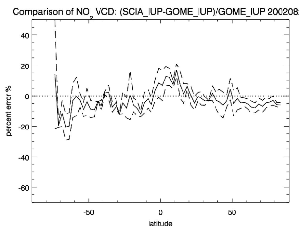
Figure 10 – Percent relative difference between SCIAMACHY and GOME total \text{NO}_2 processed by IUP, along 2 orbits on August 23, 2002, plotted as a function of latitude.
