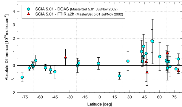
Figure 4 - Meridian variation of the mean absolute difference between near real time total nitrogen dioxide in July/November 2002 as reported by SCIAMACHY SCI_NL 5.01 and by NDSC ground-based spectrometers (SCIA-NDSC).
