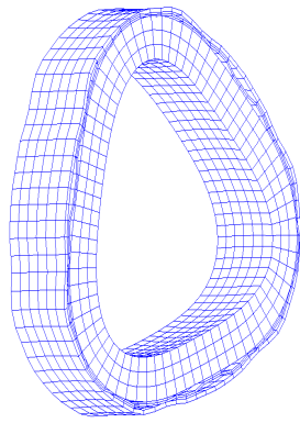
(a) Mode 35, 3640 Hz
