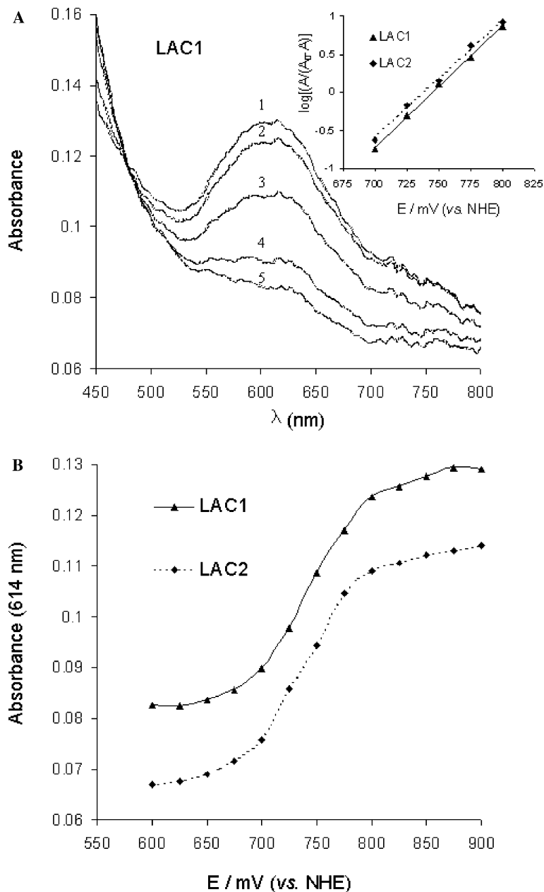
Fig. 1. Mediated spectroelectrochemical redox titration of two Trametes pubescens laccases using a gold capillary cell (22 \mu\text{M} LAC1 and 18 \mu\text{M} LAC2; 200 \mu\text{M} \text{K}_4\text{Mo}(\text{CN})_6 ; 0.1 M phosphate buffer, pH 6.5). (A) Absorbance spectra recorded during the redox titration of LAC1. Curves 1–5 are absorbance spectra of the enzyme at applied potentials 900, 800, 750, 700, and 600 mV, respectively. Inset: Nernstian plots of the E dependences of the absorbance at 614 nm for both laccases. (B) Spectroelectrochemical titration curves reflecting the dependence of absorbance of the laccase solution at 610 nm vs. the applied potential.
