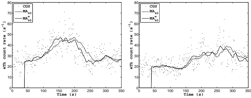
Figure 4.10: \text{MA}_{40} (thin line) and \text{MA}_{40}^w (thick line) for eTh along routes I (left) and II (right). The CGS count rate is also given, for comparison. Adapted from Paper IV.
