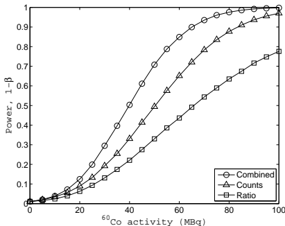
Figure 4.5: Power of the two-sided proposed test (circles) for different ^{60}\text{Co} activities. The power of the two-sided likelihood test (squares, k = 3 ) and mid-p version of S&D's test (triangles) are also given. \alpha was set to 1%. The procedure of the power test is described in detail in Paper II.
