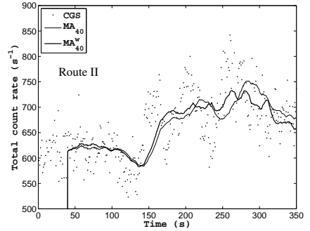
Figure 10: MA_{40}^w (thick, solid line) and MA_{40} (thin, solid line) for \text{LaBr}_3:\text{Ce} total count rate along route II.
