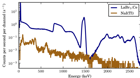
Figure 3.2: Count rates (s -1 ) of the LaBr 3 :Ce crystal (Detector system 4) and a NaI(Tl) of equal size (Detector system 2). The measurements were conducted in a shielded room with low levels of background radiation. From Nilsson et al. (2011).
