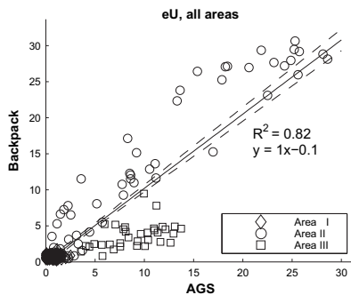
Fig. 10. Scatter plot of normalised eU samples. Dashed lines show 95% confidence interval for regression line. The regression gives unity slope and intercept close to zero, which shows a good agreement between ground and air measurements for eU.
