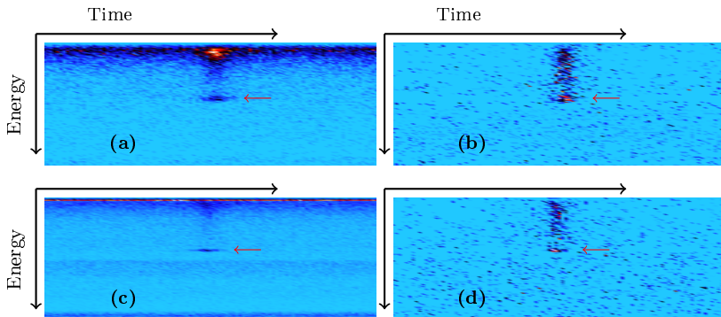
Figure 4.1: Comparison of waterfall plots (a, c) and deviation displays (b, d) for NaI(Tl) (Detector system 2, a and b) and LaBr 3 :Ce (Detector system 4, c and d) detector types. A 137 Cs point source is passed by the detectors. The primary energy of 137 Cs (662 keV) is indicated by red arrows. Note the suppressed background in the deviation displays (b, d) in general and the suppressed internal background in the LaBr 3 :Ce deviation display (d) in particular. Adapted from Nilsson et al. (2011).
