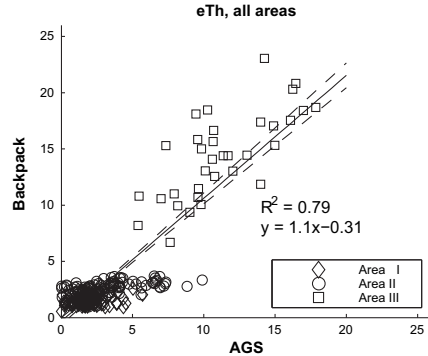
Fig. 11. Scatter plot of normalised eTh samples. Dashed lines show 95% confidence interval for regression line. A strong positive correlation exist, the straight line has an intercept and slope close to zero and unity respectively.
