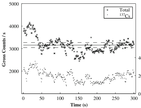
Fig. 6. Full spectrum and ^{137}\text{Cs} window gross count rates from the MOBICAL-08 exercise excerpt. The dashed lines mark the \pm 2 standard deviations about the mean (solid line) of a Poisson distribution.
