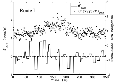
Figure 5: First derivative, f'_{AGS} , (solid line) derived from AGS data along route I after smoothing using N = 10 , cf. Eq. (3). The normalised CGS eTh counts (dots, right axis) are included for comparison.
