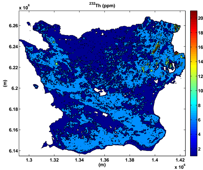
Figure 2.4: e\text{Th} concentrations for Scania from the SGU.
