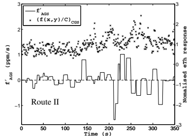
Figure 6: First derivative, f'_{AGS} , (solid line, left axis) derived from AGS data along route II after smoothing using N = 10 , cf. Eq. (3). The normalised CGS eTh counts (dots, right axis) are included for comparison.
