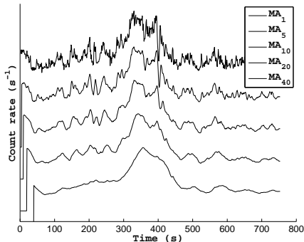
Figure 3: Illustration of the effect of different moving average lengths, N , for N = 1 (top) to N = 40 (bottom). The graphs are separated by a constant, for readability. Apart from the smoothing effect, note also how the peak position shifts as the averaging length is increased.
