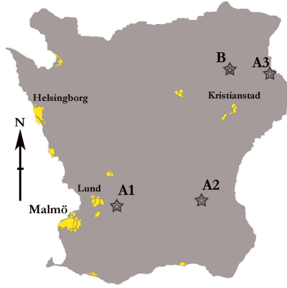
Figure 2.5: Map of Scania with the survey sites of Paper III (A1-A3) and Paper IV (B) marked. Revingehed (A1) was also the site of the experiments of Paper I and Paper V. The map was adapted from Paper III.
