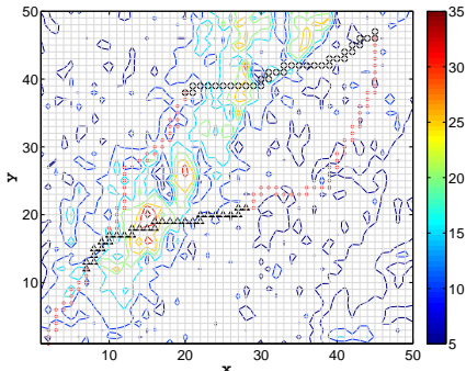
Figure 2: Contour plot of interpolated AGS eTh data (given in ppm) on a 50 \times 50 grid (cell size 180 \times 180 m 2 ). Triangles (route I) and circles (route II) mark the two CGS excerpts which pass through the area with elevated eTh levels. The rest of the roads are plotted with red dots.
