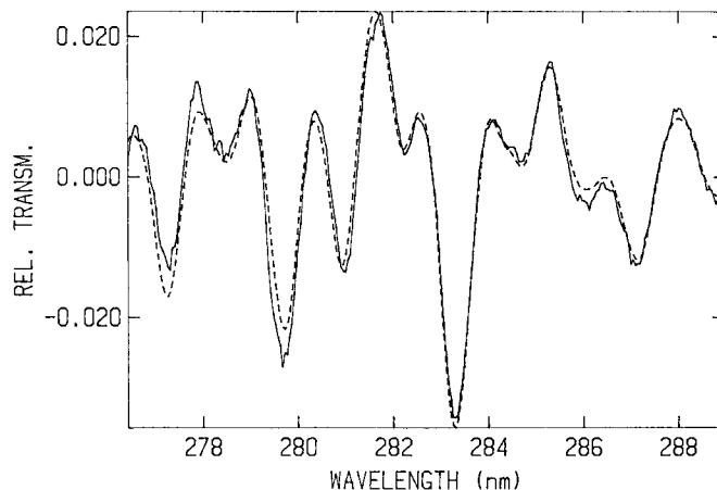
FIG. 6. Atmospheric spectrum (solid line) recorded in Lund and correlated with an O_3 and SO_2 calibration spectrum (dashed line). The spectrum corresponds to 161 \mu g/m^3 of O_3 and 2.5 \mu g/m^3 of SO_2 .
