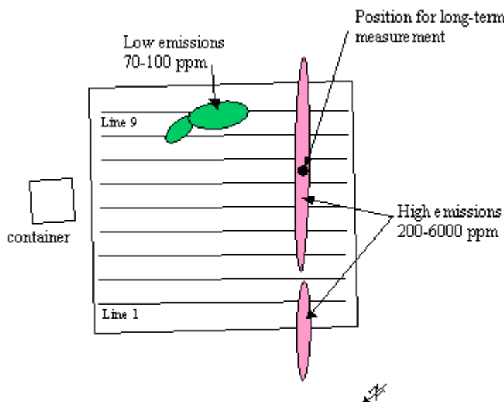
Figure 3. Laser scanning results for NSR2 test site (the orientation is the same on the previous figures, with the container placed left to the lines).
