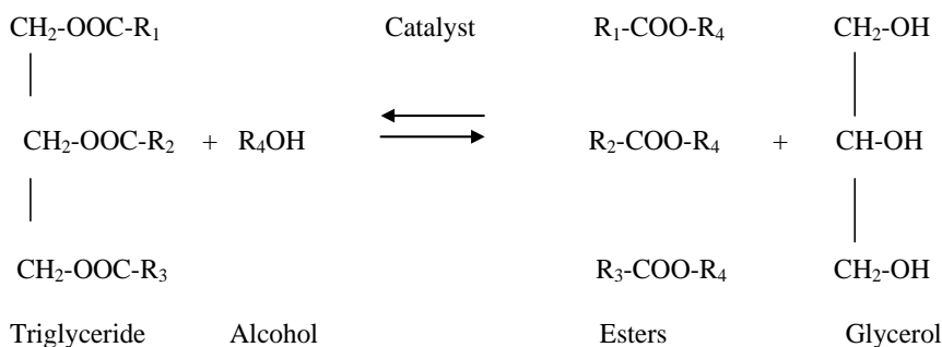
Figure 3: Triglycerides converted into esters through transesterification
