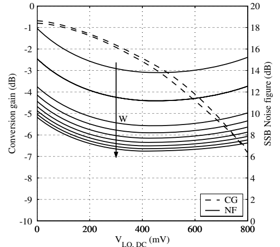
Fig. 3. Simulation of down conversion voltage gain and SSB noise figure of the quadrature LO SHM, at an IF of 10 MHz. The width is swept from 10 \mu\text{m} to 100 \mu\text{m} in steps of 10 \mu\text{m}
