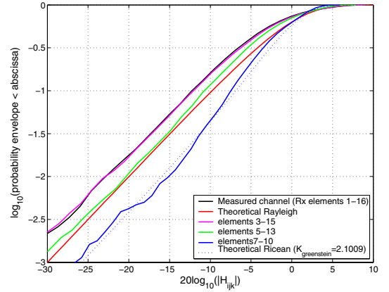
Fig. 6. Measured channel: Effect of selecting Rx elements on the fading distribution of the channel coefficients. Position Tx2Rx2336NM
