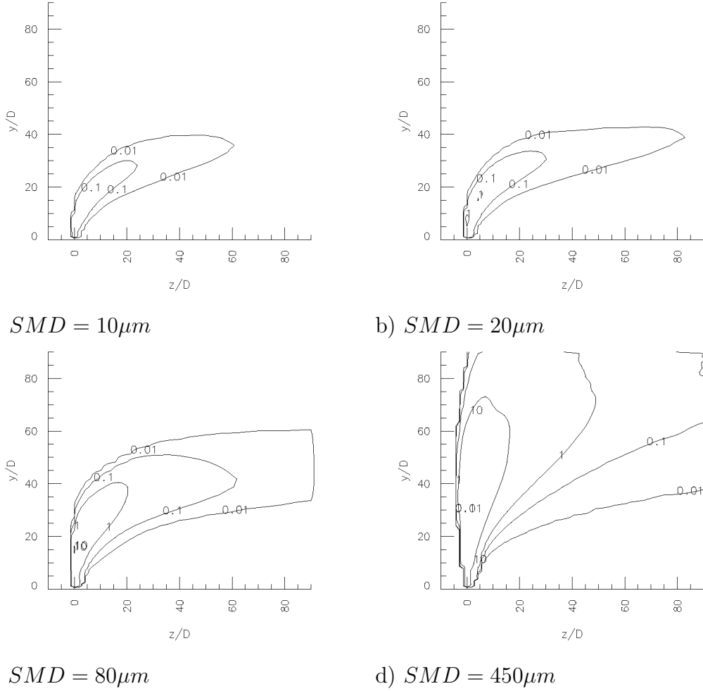
Fig. 6. Average Weber numbers for J = 41 and various injection Sauter mean diameters SMD
