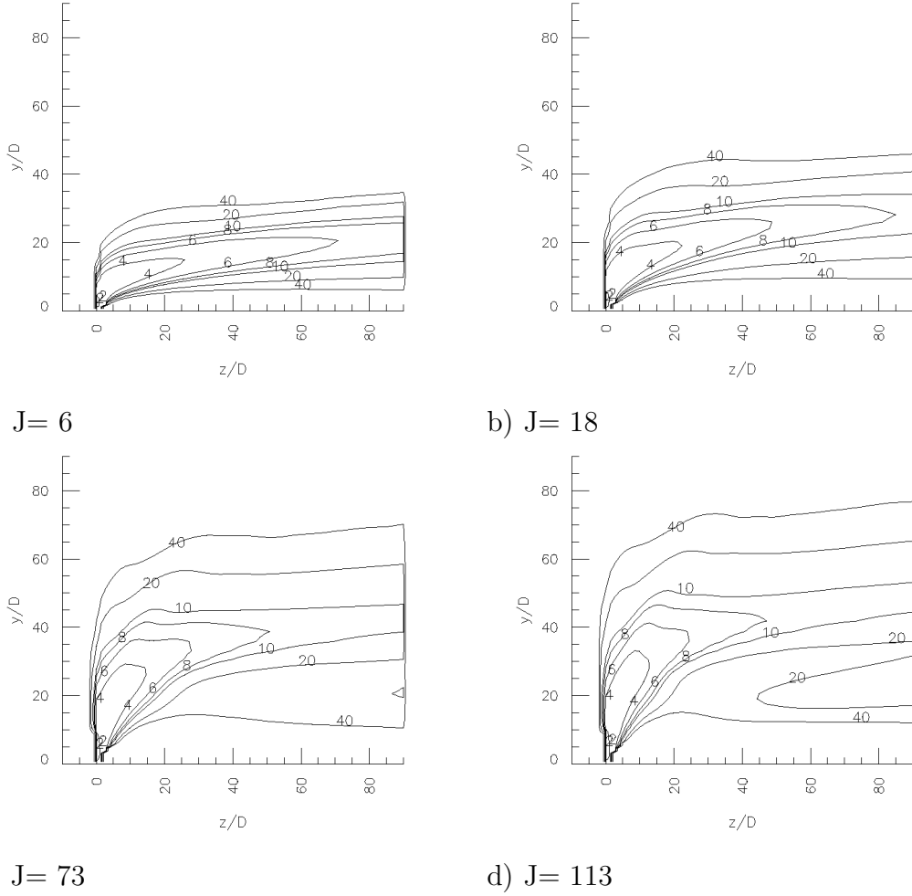
Fig. 2. Average droplet spacing for SMD = 160\mu m and various momentum flux ratios J
