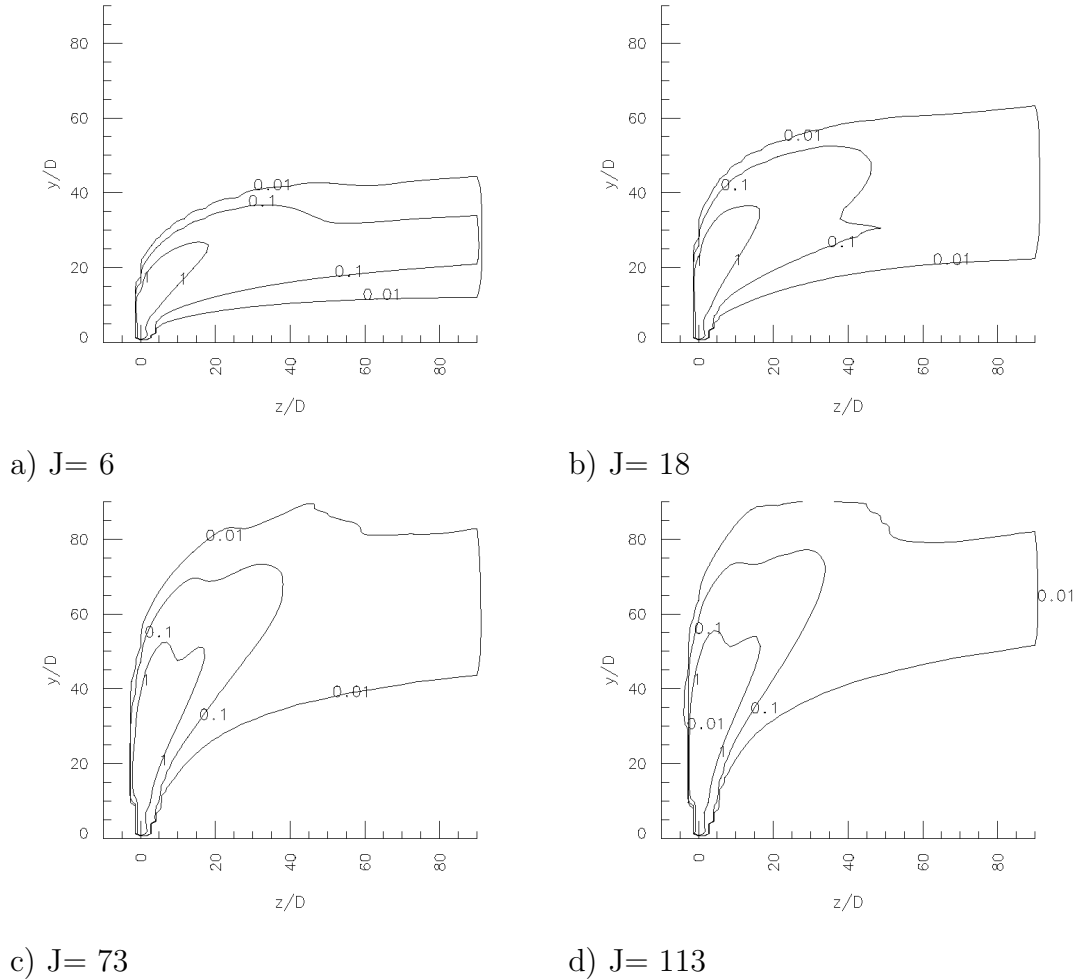
Fig. 8. Average Stokes numbers for SMD = 160\mu m and various momentum flux ratios J
