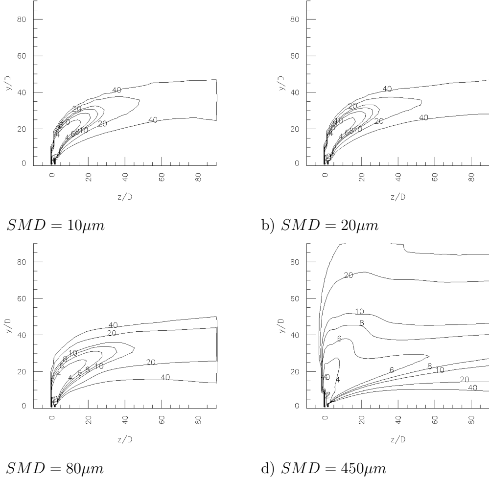
Fig. 3. Average droplet spacing for J = 41 and various injection Sauter mean diameters SMD
