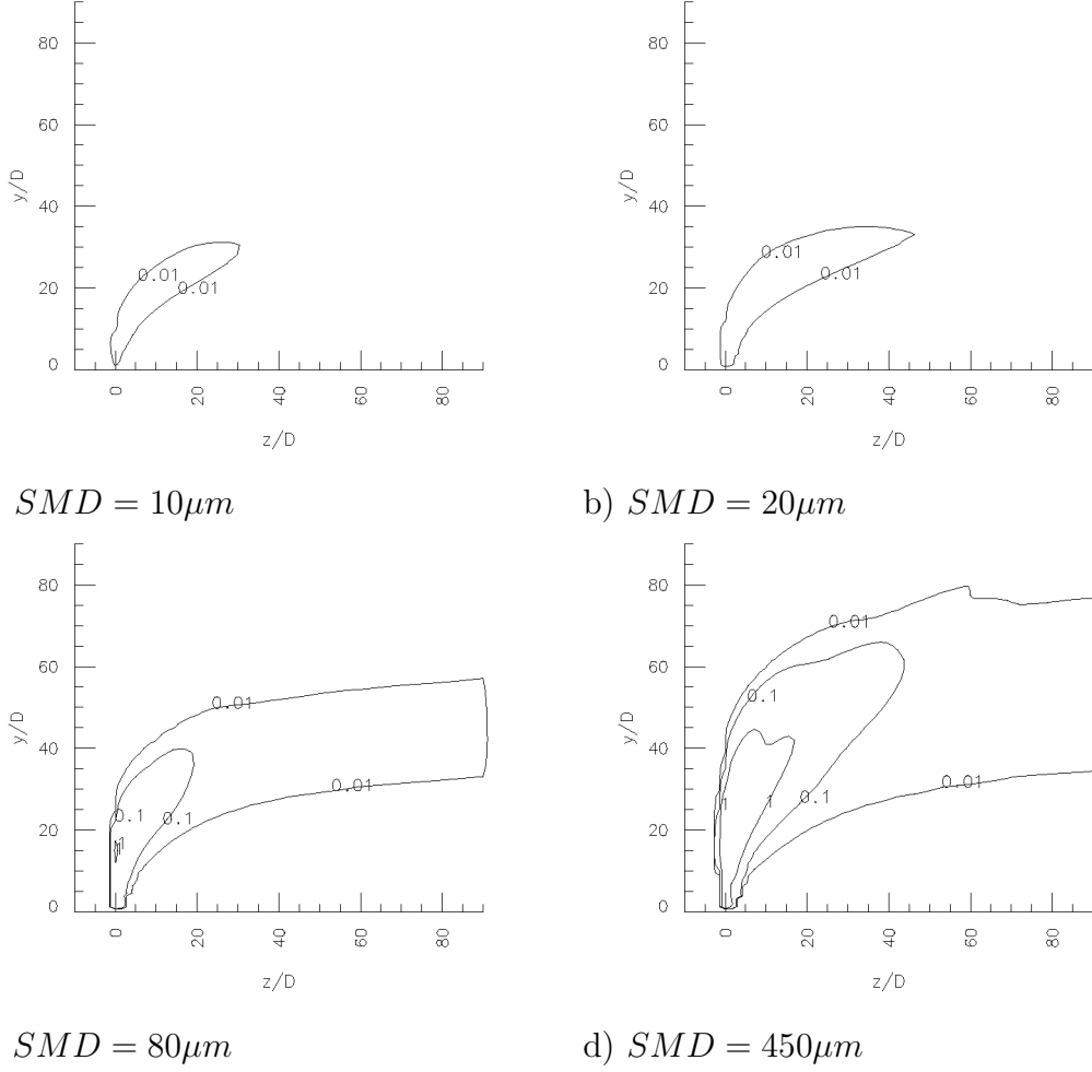
Fig. 9. Average Stokes numbers for J = 41 and various injection Sauter mean diameters SMD
