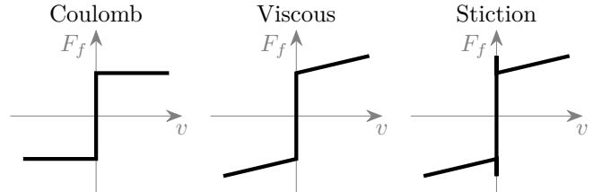
Fig. 2. Illustrations of simple friction models.
