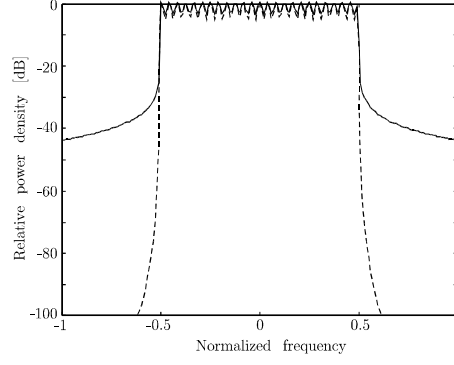
Figure 2.7: Spectrum with rectangular pulse (solid) and raised-cosine pulse (dashed).
