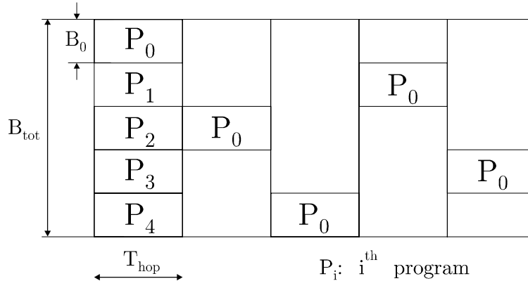
Figure 6.2: Slow frequency hopping. Each program P_i uses a bandwidth B_0 and changes frequency band after T_{\text{hop}} .
