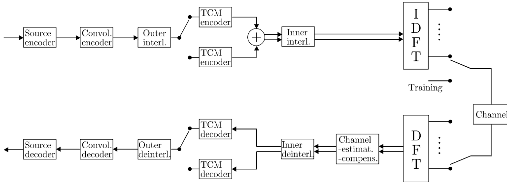
Figure 6.1: Overview of the system investigated by Höher [56].
