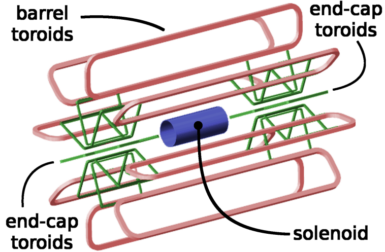
Figure 11: The ATLAS magnet system [47].
