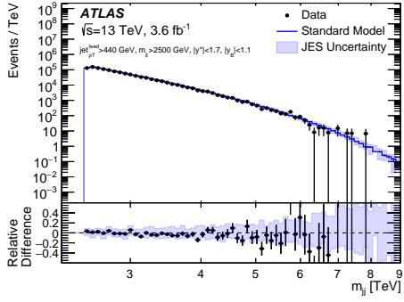
(c) m_{jj}
