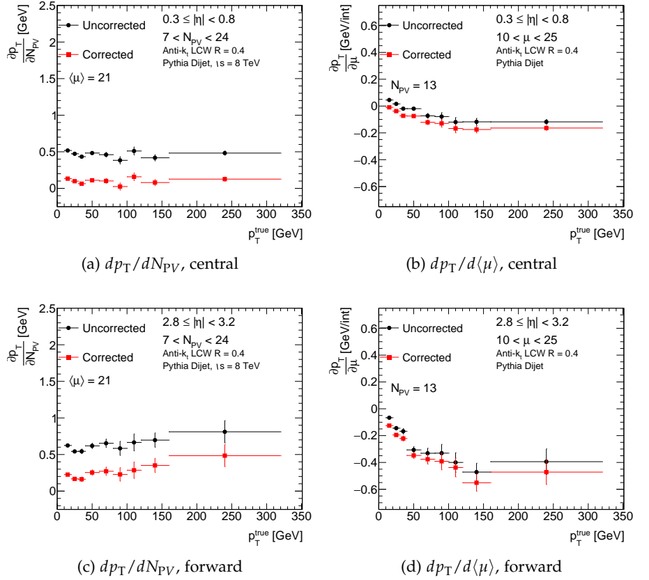
Figure 30: The dependence of p_T on (a),(c) N_{PV} and (b),(d) \langle\mu\rangle , as function of p_T , before and after \rho \cdot A subtraction, for jets clustered with anti- k_r , R = 0.4 . The top row shows central |\eta| and the bottom more forward.
