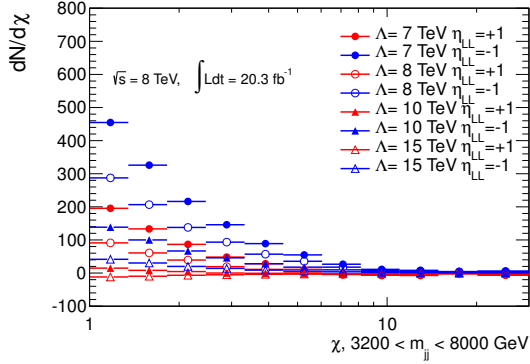
Figure 51: \chi distributions of signal with NLO K -factor applied for various \Lambda scales.
