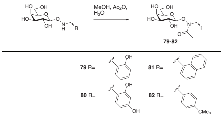
Scheme 4. Synthesis of acetylated hydroxylamines 79-82 in quantitative yields.
