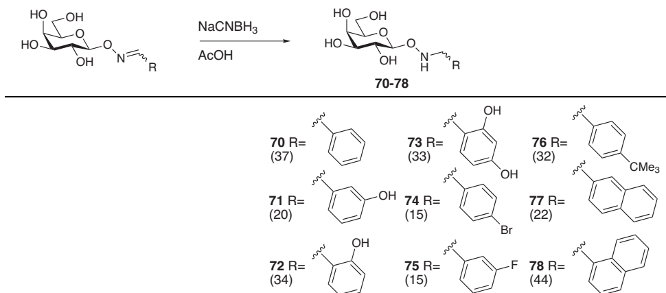
Scheme 3. Synthesis of hydroxylamines 70-78 . (Yield) in %.
