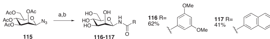
Scheme 8. Synthesis of amide analogues 116 and 117 : a) i. Pd/C, H 2 , EtOH ( 116 ) or THF ( 117 ), 200 psi, 75 minutes. ii. Acid chloride, CH 2 Cl 2 ( 116 ) or THF ( 117 ), pyridine, over night; b) MeOH, NaOMe.
