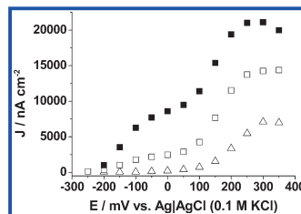
Figure 4. Polarization curves of PEI/graphite electrodes modified with MtCDH containing both the \text{CYT}_{\text{CDH}} (squares ◼, ◼) or only the \text{DH}_{\text{CDH}} domain (Δ) at pH 8 in the presence (filled symbol) or absence of 50 mM \text{CaCl}_2 (empty symbols). The responses of the modified graphite electrodes were investigated with flow injection analysis with 5 mM lactose as substrate.
