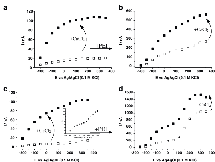
Fig. 8 Variation of response current ( I ) with the applied potential ( E ) of spectrographic graphite electrodes modified with Myriococcum thermophilum CDH (a, c) and optionally pre-modified with polyethylenimine (PEI) (b, d) in 50 mM sodium acetate buffer pH 5.5 (a, b) or 50 mM TRIS pH 8.0 (c, d) in the absence (white squares) or in the presence of 50 mM \text{CaCl}_2 (black squares) with 5 mM lactose as substrate. The inset in c shows a magnification of the response curve
