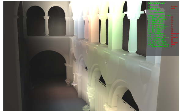
Figure 5: The sponza scene rendered using only indirect illumination and without any diffuse texturing. Note that the indirect lighting has been slightly exaggerated in this image.
