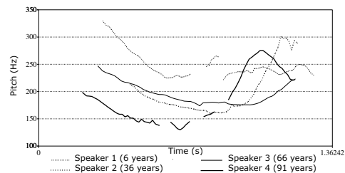
Figure 1: F 0 contours for [ʃjɛ:lən] for the four speakers.
