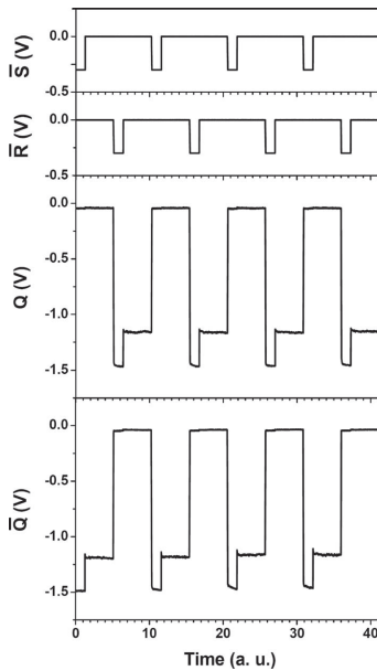
FIG. 3. Measured SR latch functionalities of the device. The high and low logic states of the inputs ( \bar{S} and \bar{R} ) were set to be 0 and -0.3 V, while those of the outputs ( Q and \bar{Q} ) were to be -0.04 and \approx -1.2 V.
