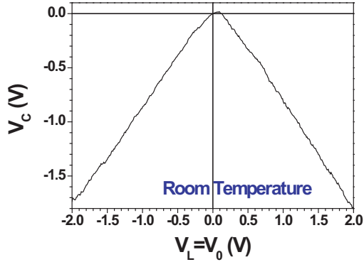
Figure 4.4: The no-load central branch output V_C as a function of V_0 measured at room temperature for the device shown in Figure 4.3 (push-pull fashion).
