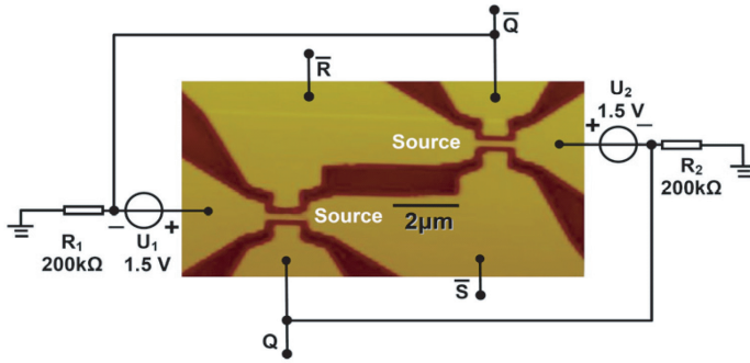
Figure 3.7: An AFM image of the integrated SR latch device made on an In-GaAs/InP wafer 4113, where the dark parts correspond to wet etched trenches. A schematic diagram of the measurement circuit for the latch is also shown. The sources of the two in-plane gate transistors are marked with white text.
