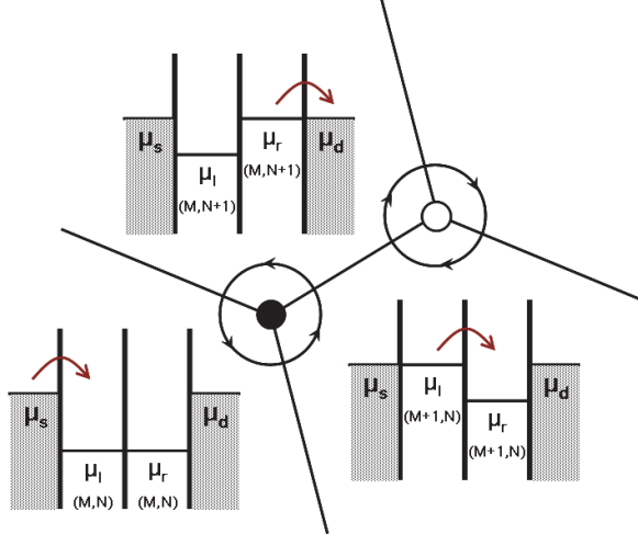
Figure 5.10: An illustration of the two kinds of triple points at the corners of the hexagons. ● and ○ correspond to the electron and hole transport processes, respectively, cf. the large circle with arrows. For the electron transfer process, the 3 degenerate charge states are schematically shown and the alignment of the QD electrochemical potentials with respect to the source and drain Fermi level is displayed. Here, the arrows indicate the motion direction of the electron.
