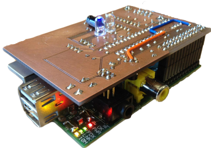
Fig. 3. A picture of the completed embedded system, the upper part (CAN-bus interpreter) is connected to the lower part (Raspberry Pi) over their respective RS-232 serial ports.
