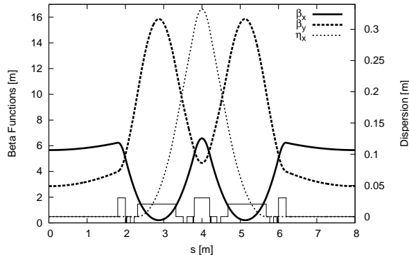
Figure 6: Beta functions \beta_x, \beta_y and dispersion \eta_x for one achromat of the MAX IV 1.5 GeV storage ring. The position of the dipoles, combined quadrupole/sextupole magnets, and discrete sextupoles are indicated at the bottom.
