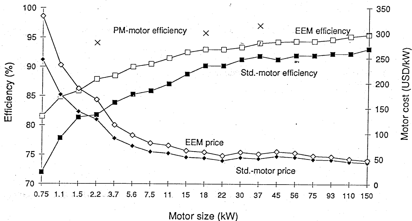
Fig. 2. Full load efficiencies and wholesale prices of standard and energy-efficient 3-phase motors in Canada as a function of rated output capacity [6]. Also shown are reported efficiencies of permanent magnet motors [29,30,31].
