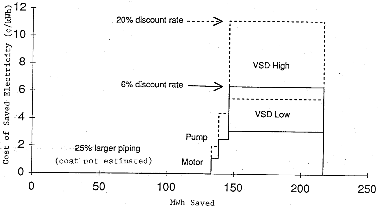
Fig. 16. Pumping electricity conservation-supply curves showing potential electricity savings and costs of saved electricity for the variable-flow application described by Table 3 and Fig. 11, with the duty cycle and input power requirements as shown in Fig. 13a and 15, respectively. Graph (a) assumes no modifications are made to the piping, in which case a 75-kW motor is required. Graph (b) assumes 25% larger diameter piping, in which case a 45-kW motor can be used. The extra costs for the more efficient motors are from Fig. 2. The extra cost for more efficient pumps is assumed to be 20% of the cost for a standard pump, based on [1]. Standard pumps are assumed to cost $9000 for the 75-kW unit [18] and $7220 for a 45-kW unit. VSD equipment costs are from the lower curve in Fig. 4b. These are combined with the high and low installation costs from Fig. 4a to give the two cost-of-saved-electricity estimates here. Costs for larger diameter piping were not estimated. The calculations assume 5000 operating hours per year and 10-year equipment lifetime.
