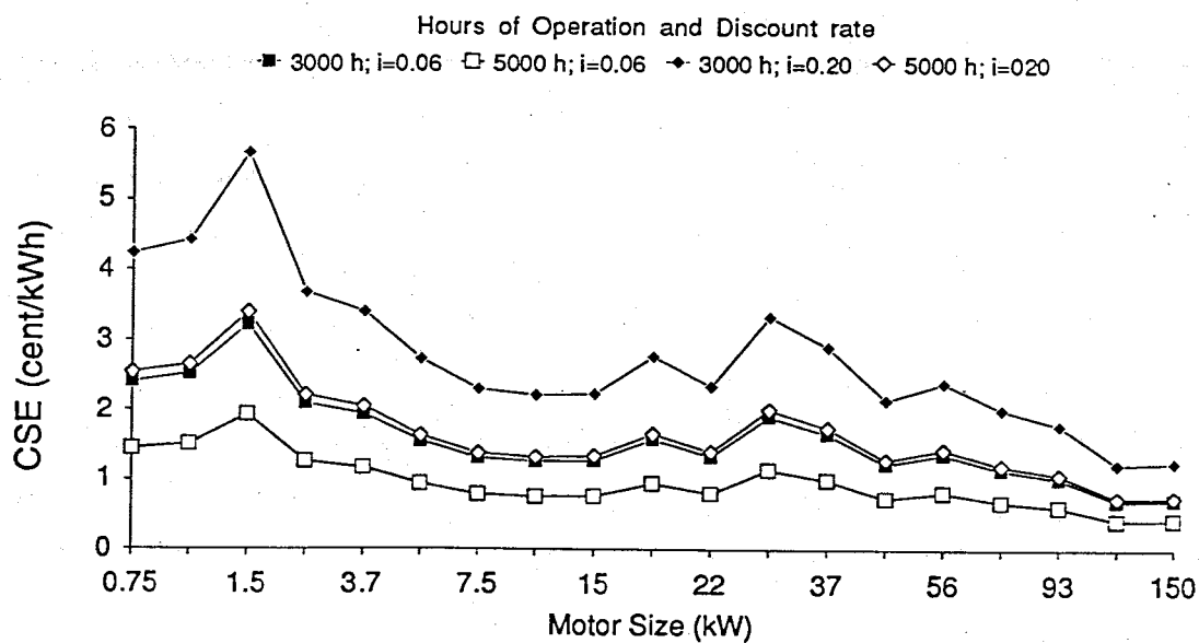
Fig. 3. Calculated cost-of-saved-electricity for new investments in energy-efficient motors versus standard motors. Motor costs and performance are from Fig. 2. A 10-year economic lifetime is used in all cases.
