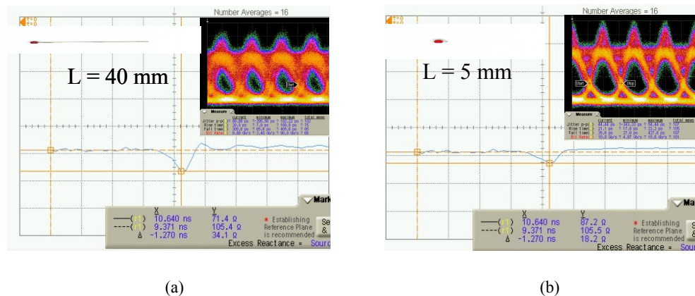
Fig. 2. (a) Processing board with long interconnects. (b) Processing board with short interconnects.
