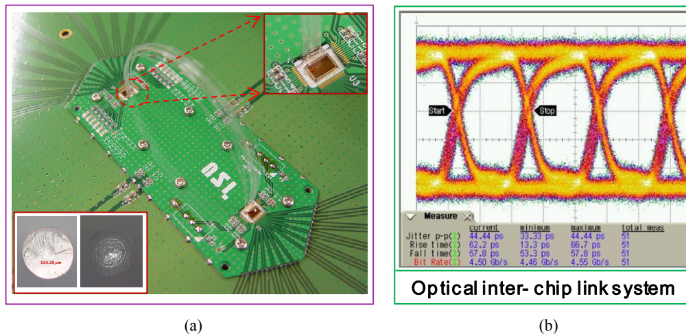
Fig. 7. (a) Inter-chip link system with an optical link. (b) Eye-diagram measured for 4.5 Gbp/s transmission of a 2^{31}-1 PRBS NRZ data.
