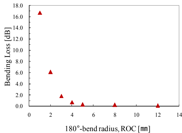
Fig. 4. The bending loss of the POF as a function of radius of curvature (ROC).
