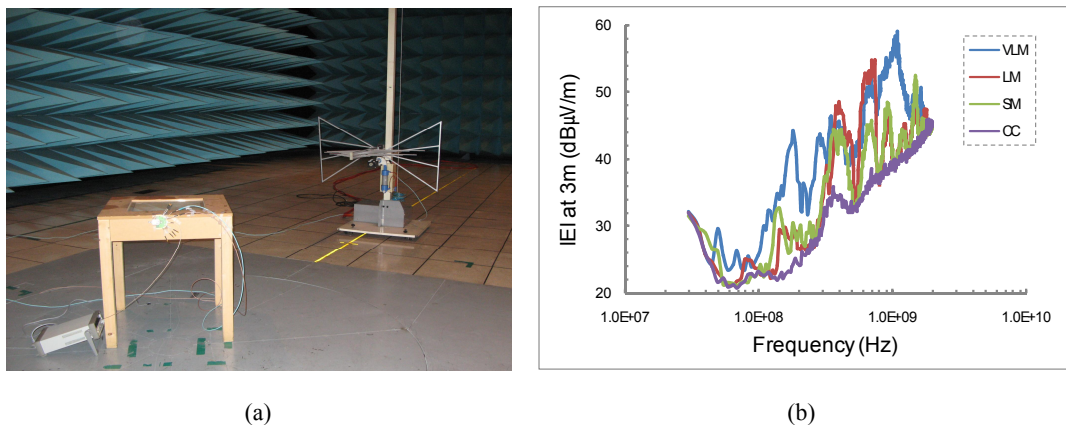
Fig. 6. (a) EMI test set-up, (b) EMI characteristics of optical modules.
