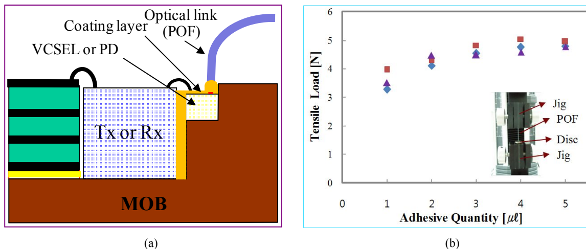
Fig. 5. (a) Structure of metal optical bench. (b) Test of tensile strength for UV epoxy.
