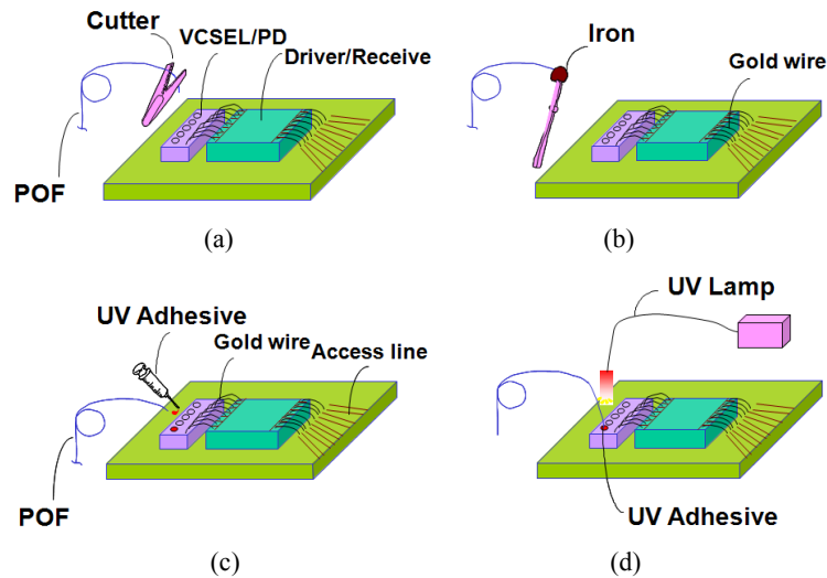
Fig. 3. Packaging process for an optical alignment and coupling between VCSELs and optical wiring link (POF).
