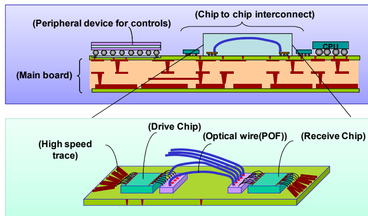
Fig. 1. Architecture of an optical link system using an optical wiring link block.
